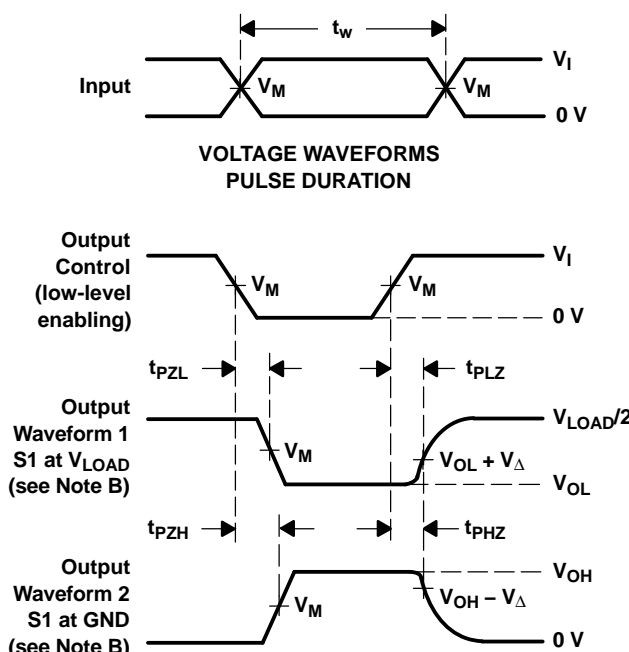
VOLTAGE WAVEFORMS ENABLE AND DISABLE TIMES
