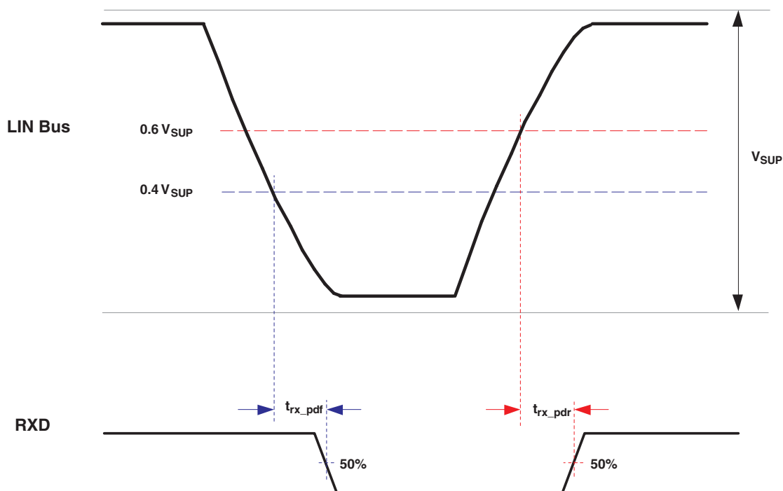
Figure 6. Propagation Delay
