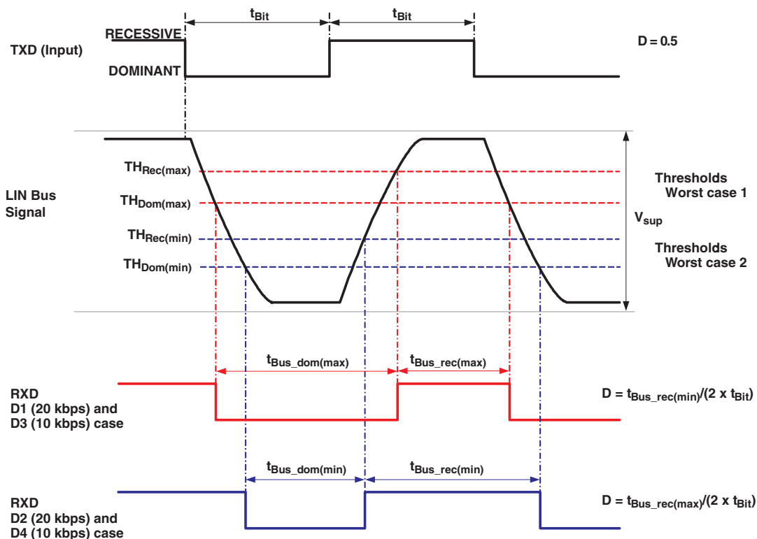
Figure 5. Definition of Bus Timing Parameters
