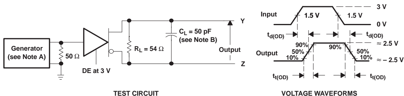
TEST CIRCUIT
