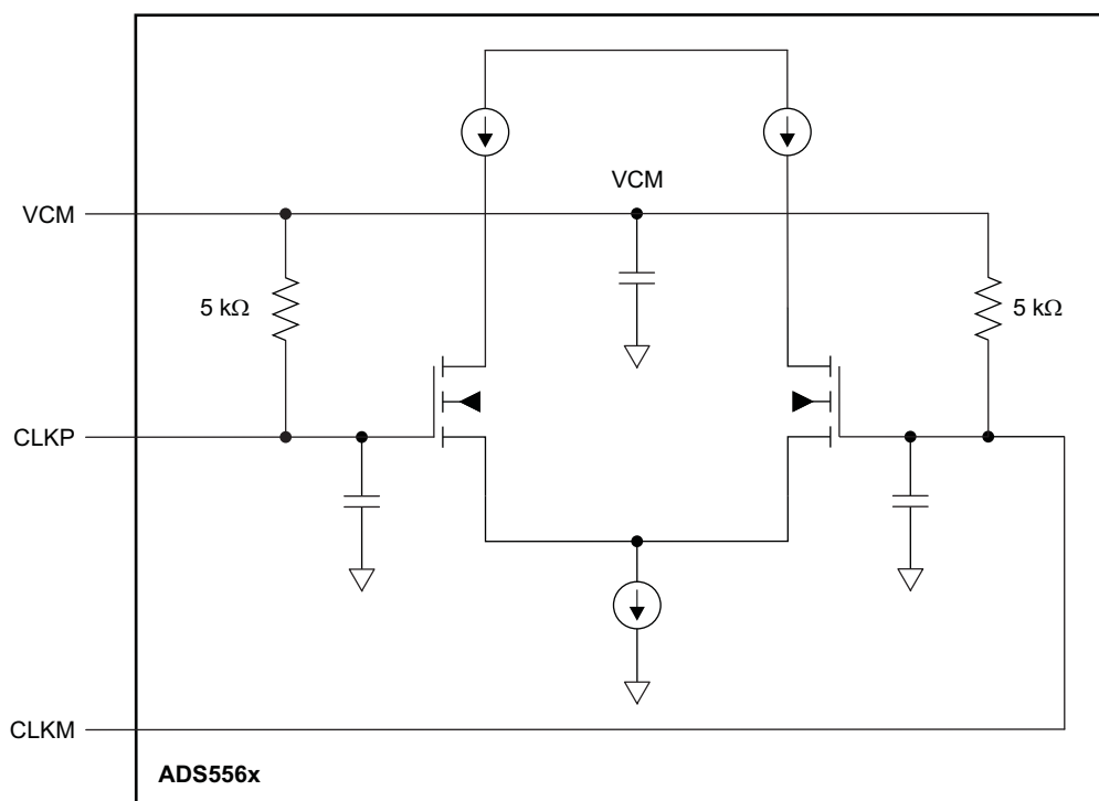
Figure 54. Clock Inputs
