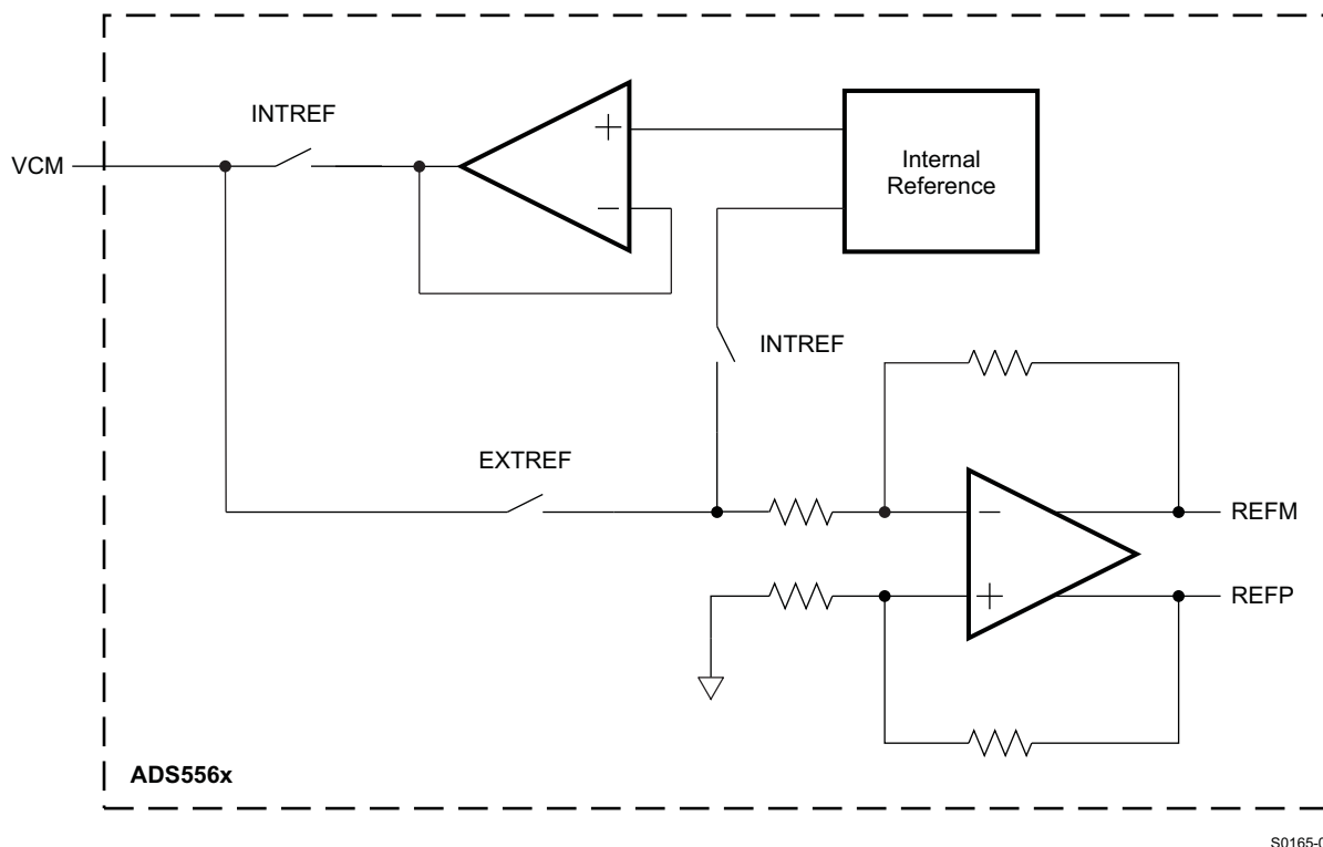
Figure 50. Reference Section
