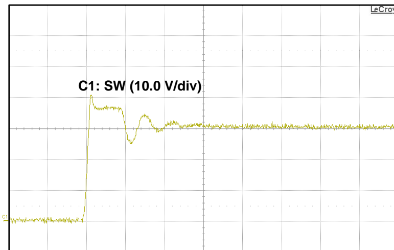
Figure 12. SW Pin Voltage Overshoot
