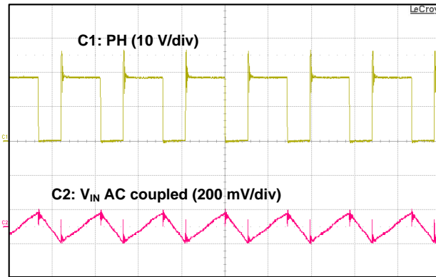
Figure 10. Input Voltage Ripple
