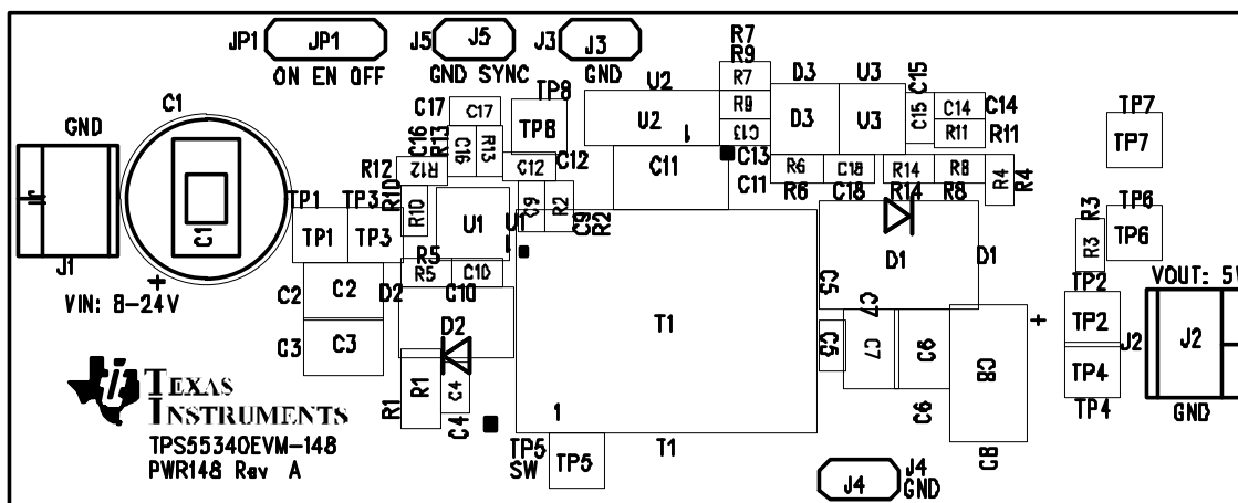
Figure 17. Top-Side Assembly and Silk
