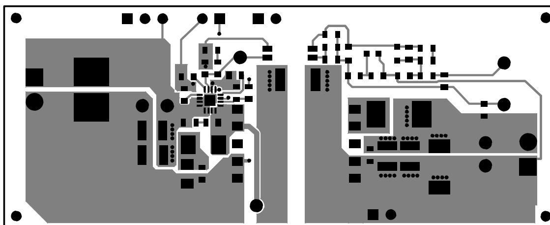
Figure 18. Top-Side Layout
