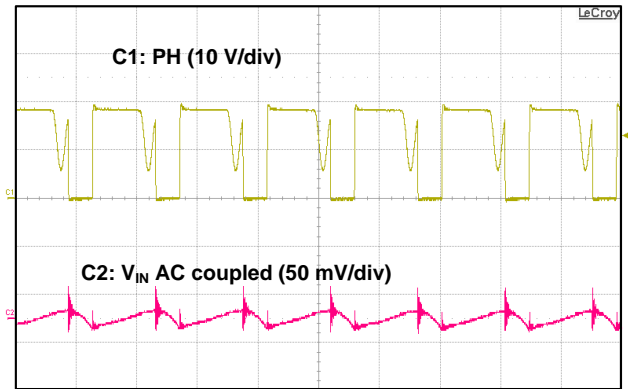
Figure 11. DCM Input Voltage Ripple
