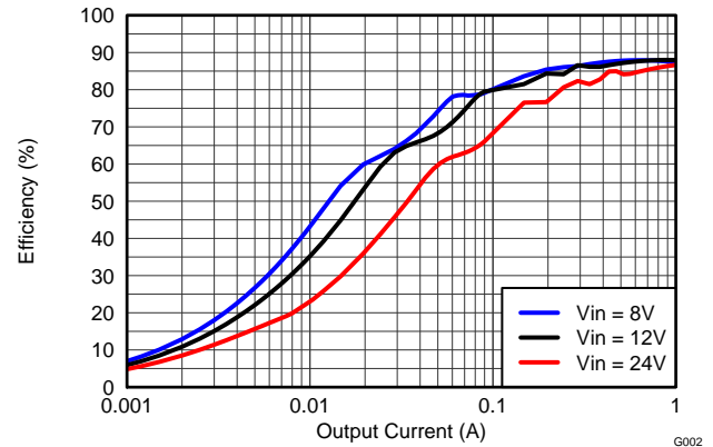
Figure 2. Light-Load Efficiency
