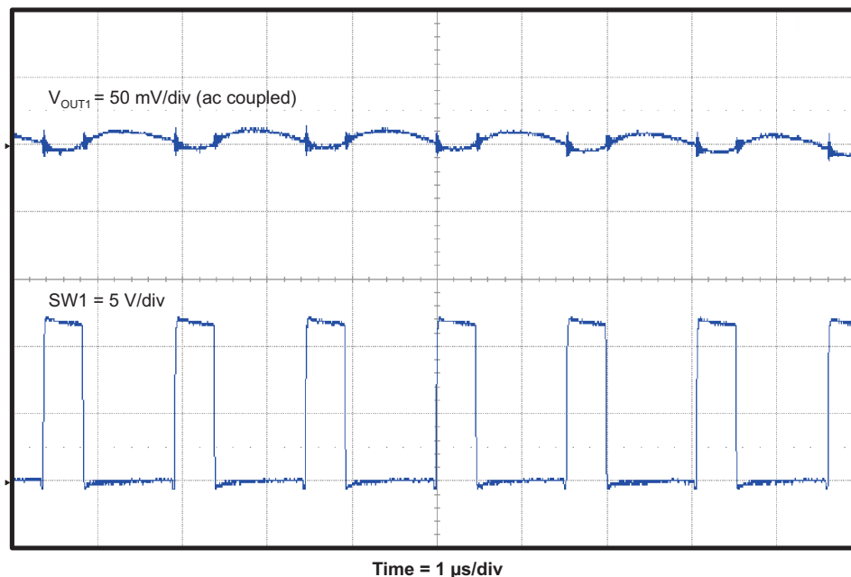
Figure 11. TPS54394EVM Converter 1 Output Voltage Ripple
