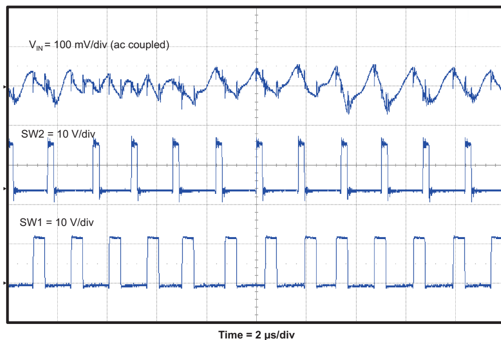
Figure 15. TPS54394EVM Input Voltage Ripple
