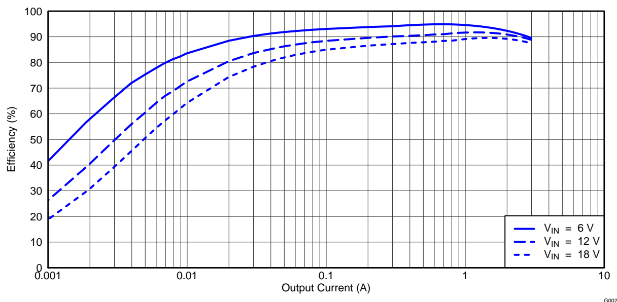
Figure 2. TPS54394EVM Converter 1 Light Load Efficiency
