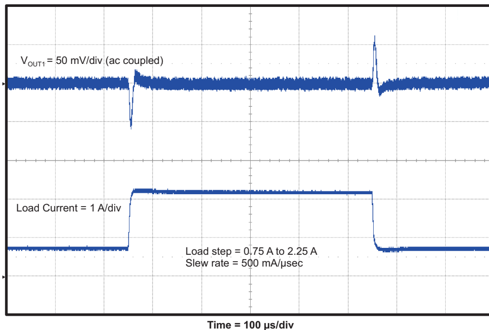
Figure 9. TPS54394EVM Converter 1 Load Transient Response
