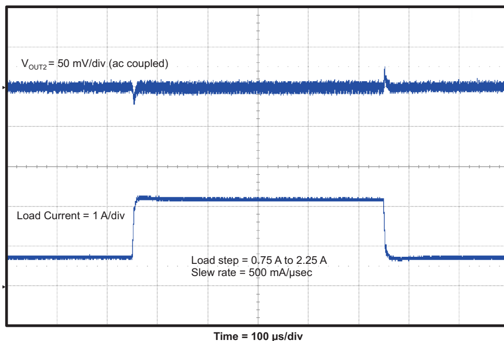
Figure 10. TPS54394EVM Converter 2 Load Transient Response
