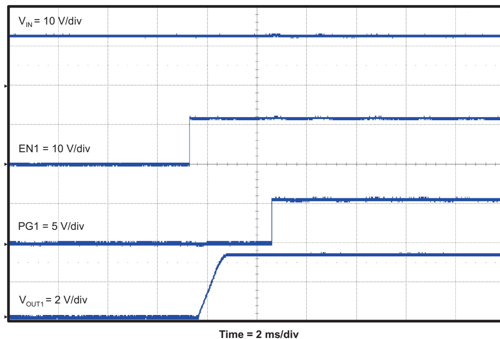
Figure 17. TPS54394EVM Start-Up Relative to EN1
