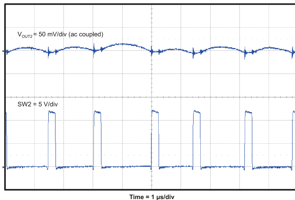
Figure 13. TPS54394EVM Converter 2 Output Voltage Ripple
