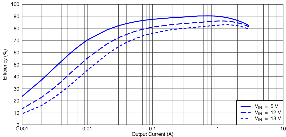
Figure 4. TPS54394EVM Converter 2 Light Load Efficiency
