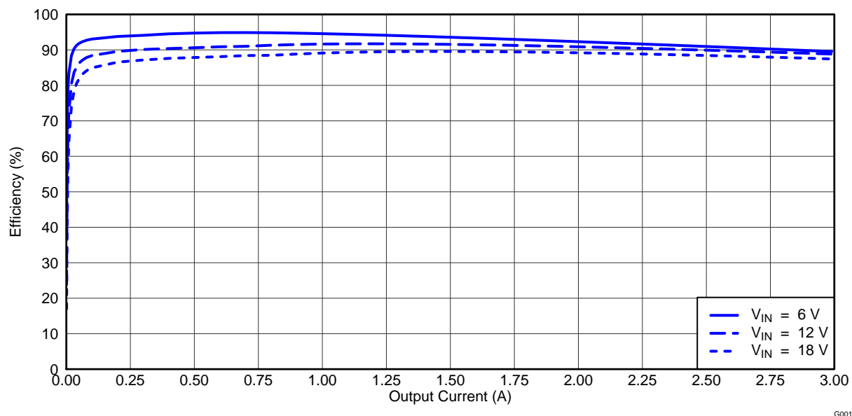
Figure 1. TPS54394EVM Converter 1 Efficiency
