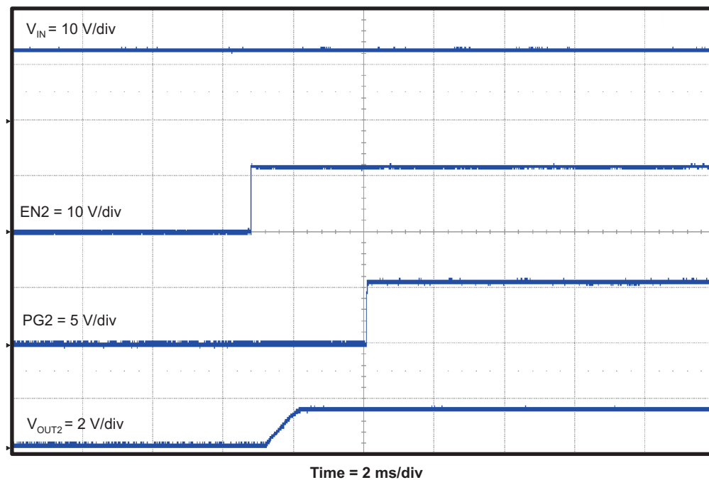
Figure 19. TPS54394EVM Start-Up Relative to EN2
