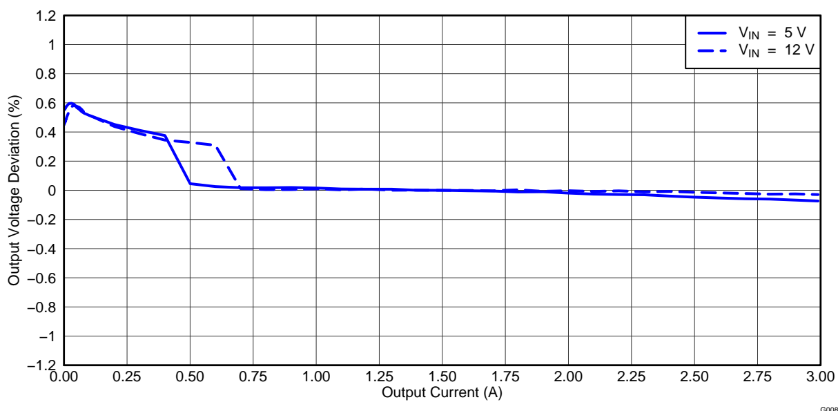
Figure 6. TPS54394EVM Converter 2 Load Regulation
