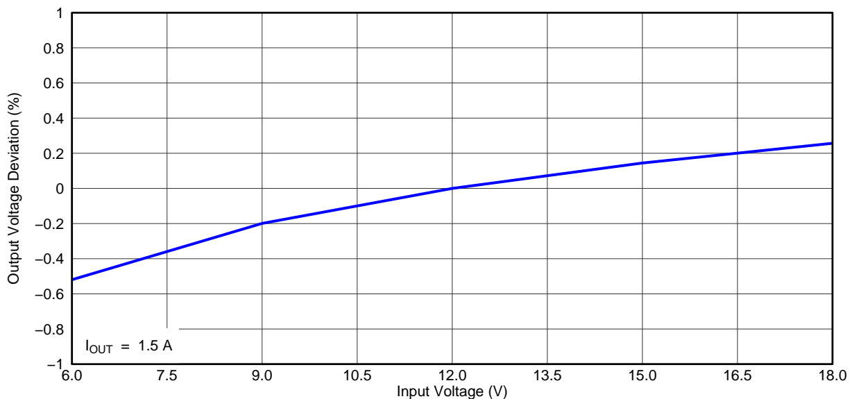
Figure 7. TPS54394EVM Converter 1 Line Regulation
