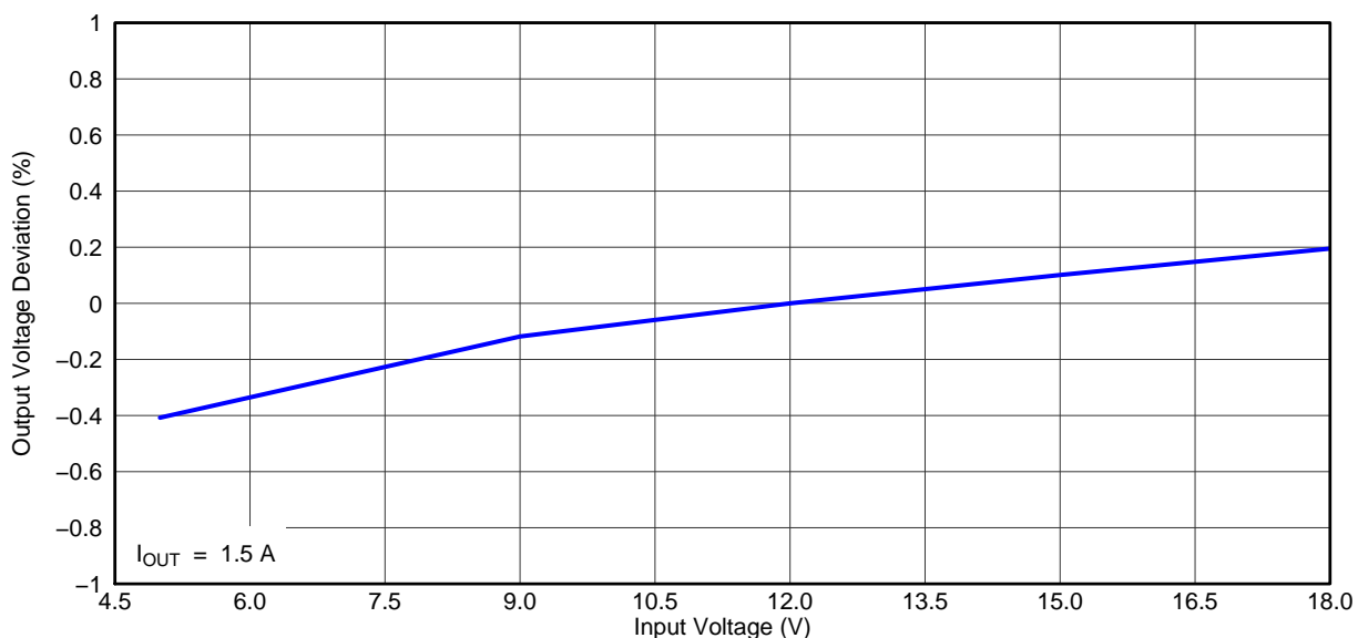
Figure 8. TPS54394EVM Converter 2 Line Regulation
