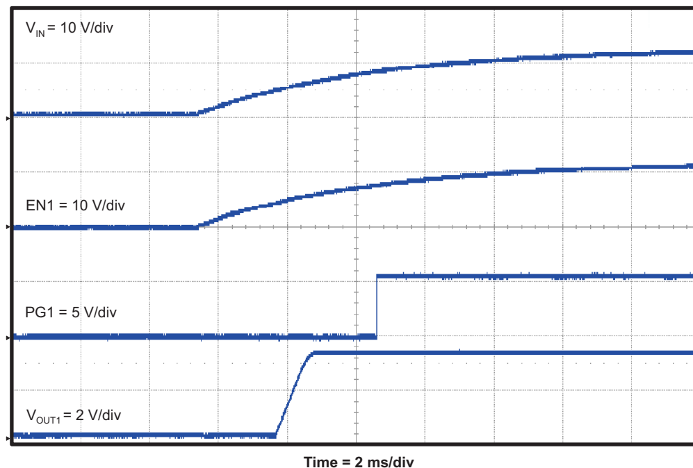
Figure 16. TPS54394EVM Converter 1 Start-Up Relative to V_{IN}
