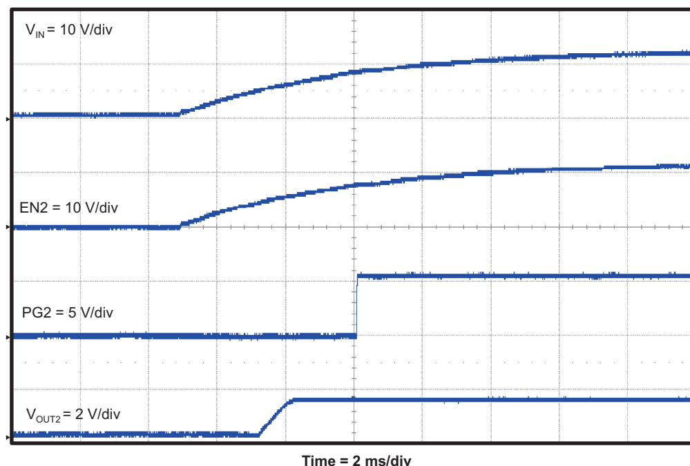
Figure 18. TPS54394EVM Converter 2 Start-Up Relative to V_{IN}
