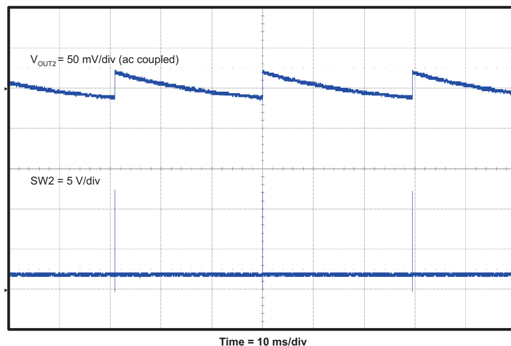
Figure 14. TPS54394EVM Converter 2 Eco-mode™ Output Voltage Ripple at No Load
