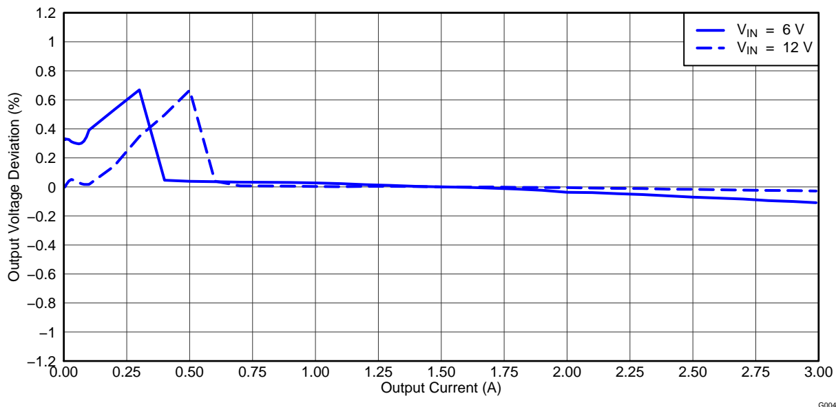
Figure 5. TPS54394EVM Converter 1 Load Regulation
