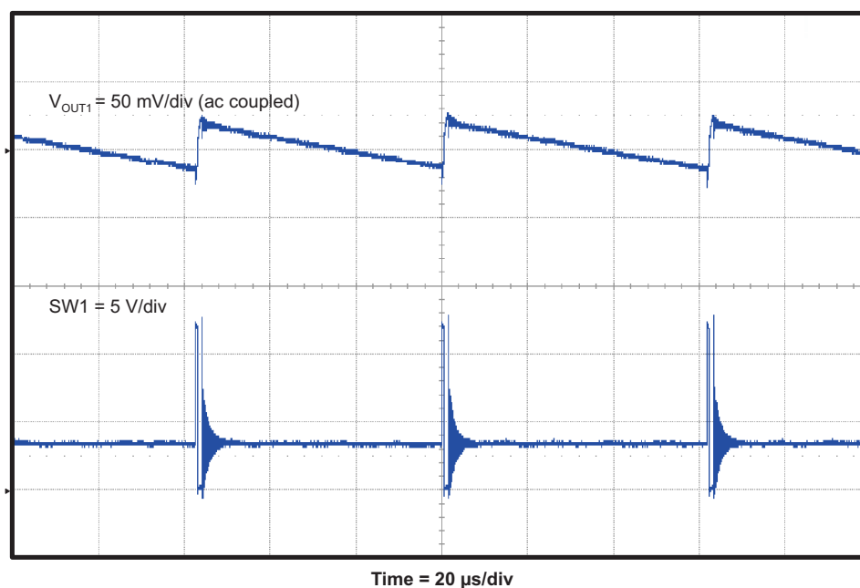
Figure 12. TPS54394EVM Converter 1 Eco-mode™ Output Voltage Ripple at No Load
