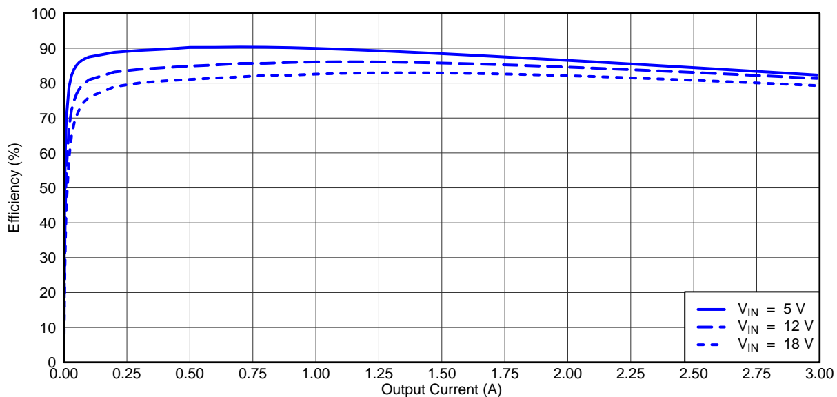
Figure 3. TPS54394EVM Converter 2 Efficiency
