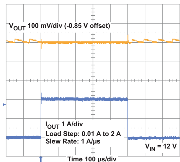
Figure 7. TPS54428EVM-052 Load Transient Response, 0.01 A to 2 A
