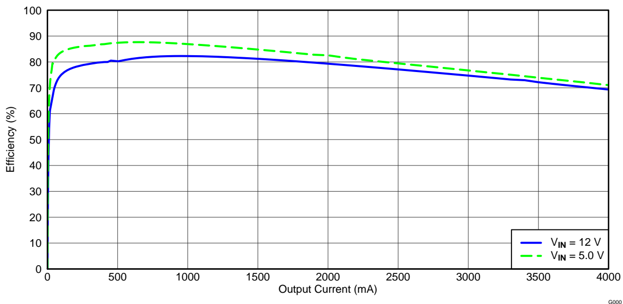
Figure 1. TPS54428EVM-052 Efficiency
