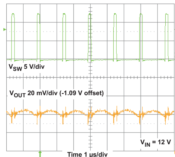
Figure 8. TPS54428EVM-052 Output Voltage Ripple
