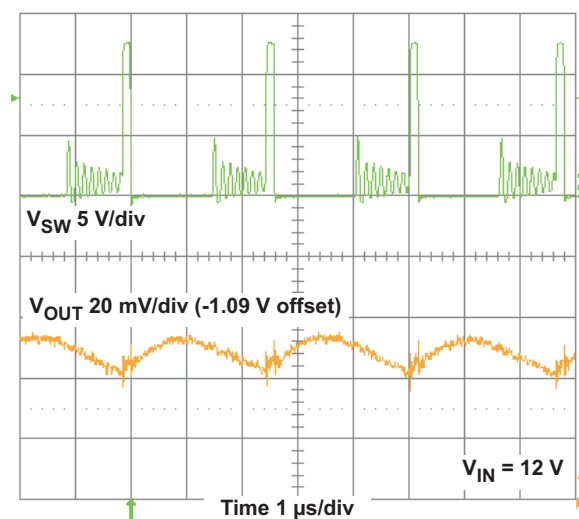
Figure 9. TPS54428EVM-052 Eco-mode™ Output Voltage Ripple
