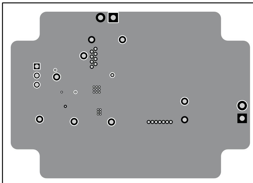
Figure 19. Internal Layer 2
