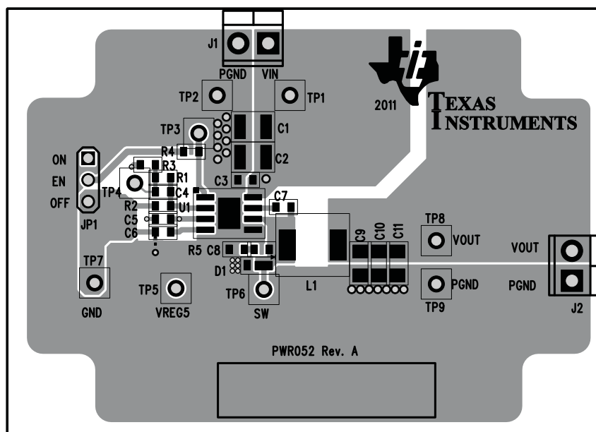
Figure 16. Top Assembly
