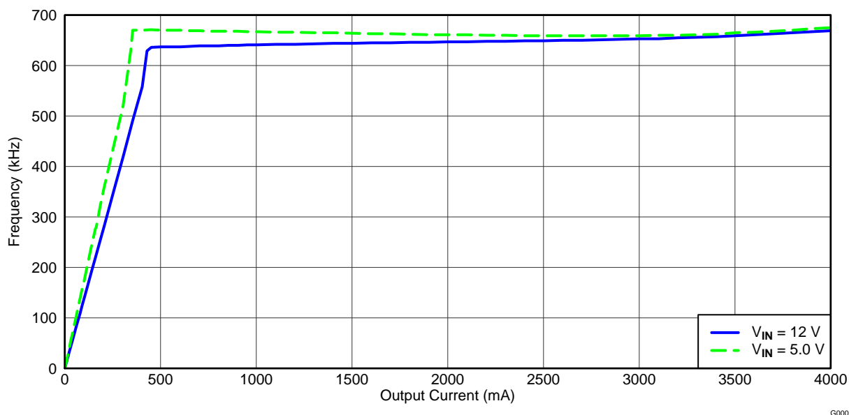
Figure 5. TPS54428EVM-52 Frequency
