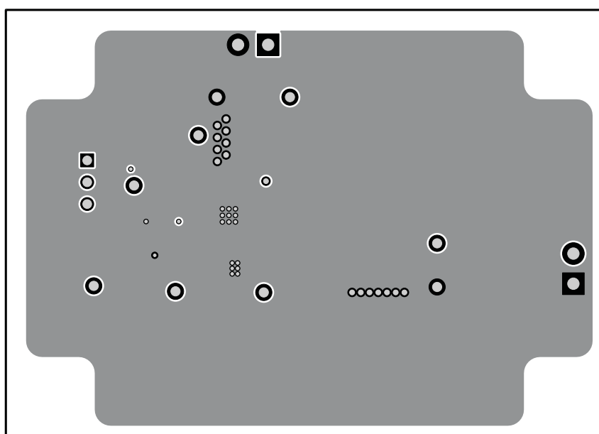
Figure 18. Internal Layer 1
