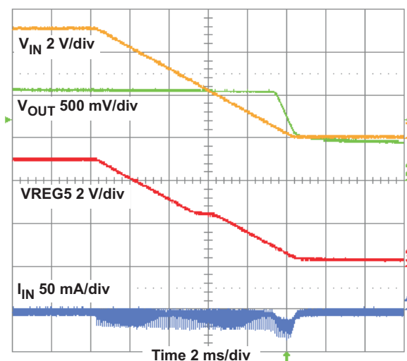
Figure 13. TPS54428EVM-052 Shut-down Relative to V_{IN}
