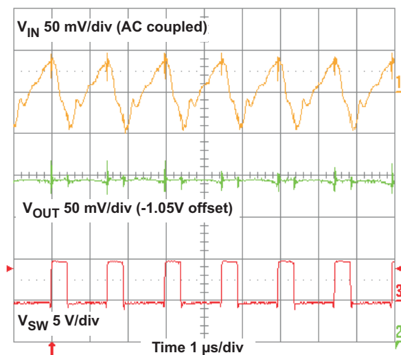
Figure 11. TPS54428EVM-052 Input Voltage Ripple
