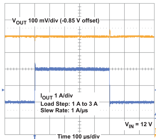
Figure 6. TPS54428EVM-052 Load Transient Response, 1 A to 3 A
