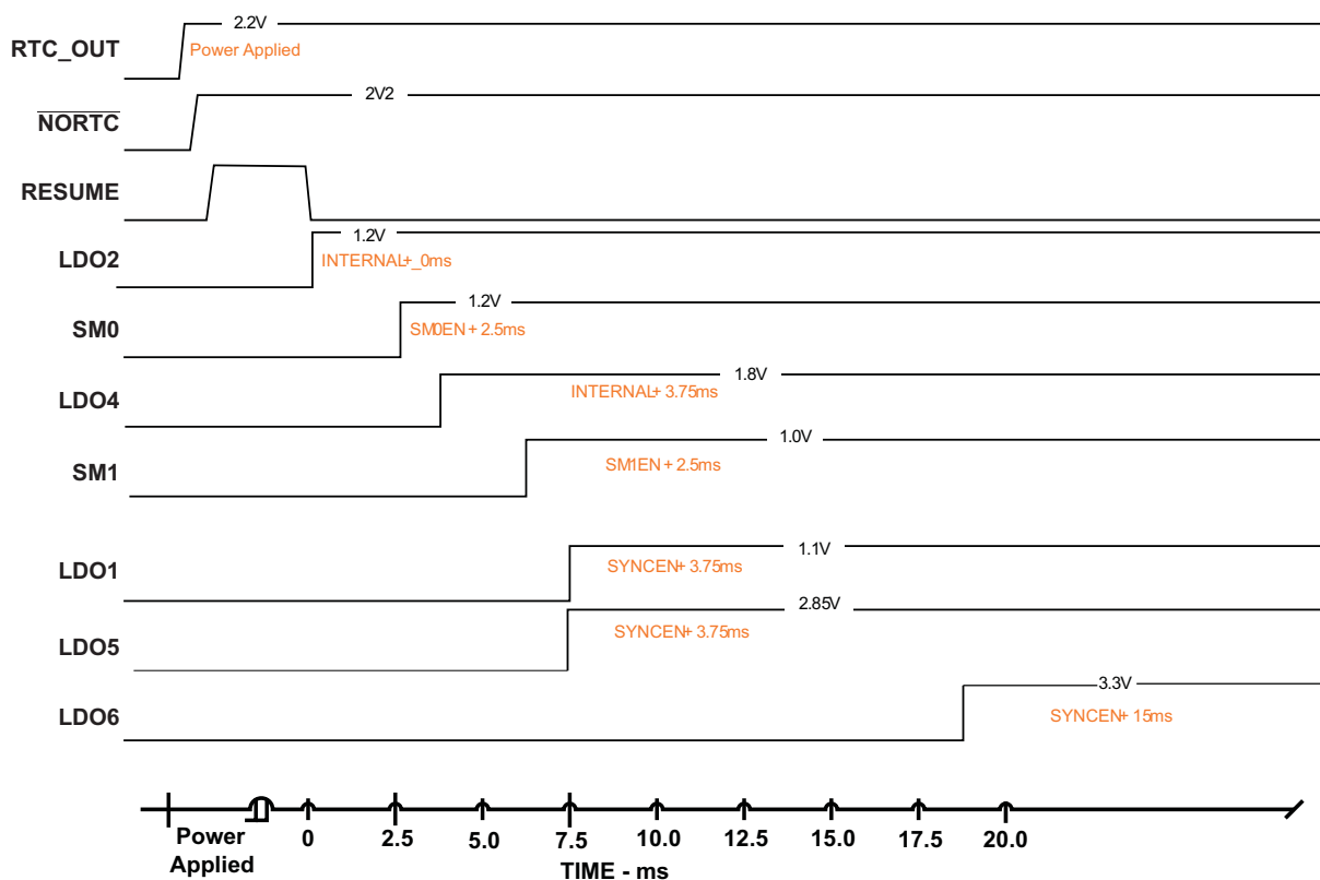
Figure 4-5. Sequence Timing
