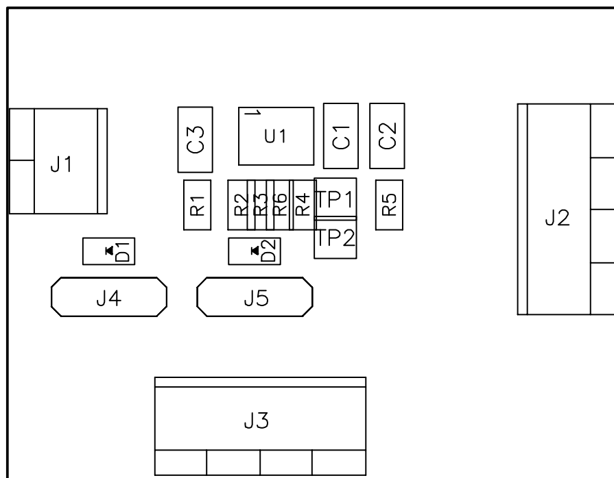
Figure 3–2. Assembly View
