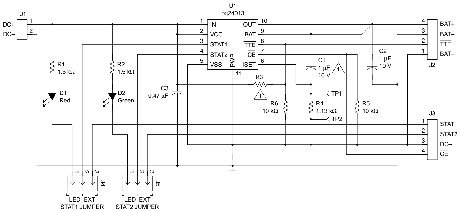
Figure 3–1. EVM Schematic Diagram
