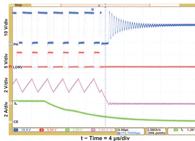
Figure 5. Charge Disable
