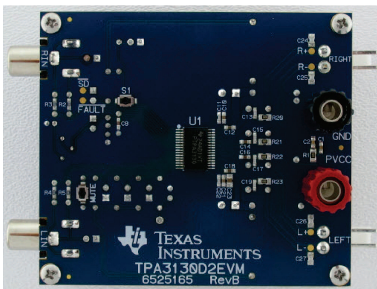
Figure 1. TPA3130D2EVM Top Photo
