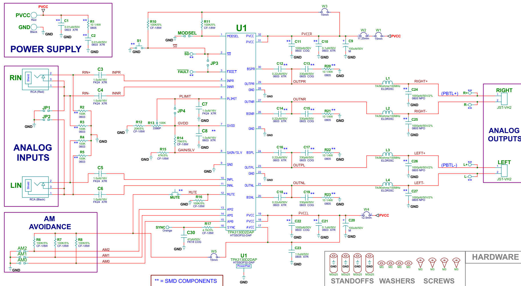
Figure 3. TPA3130D2EVM Schematic
