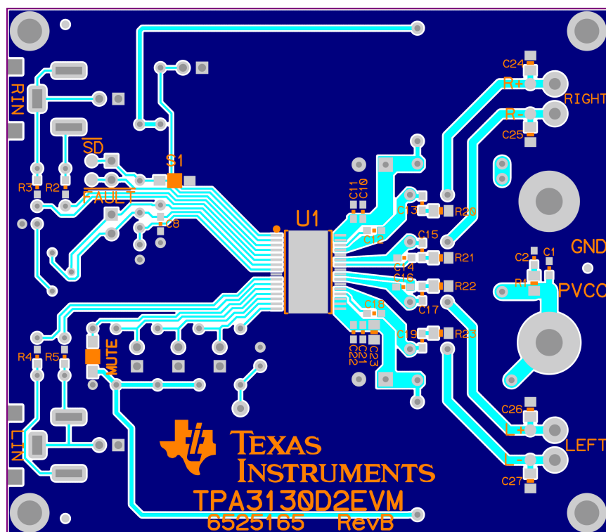
Figure 4. TPA3130D2EVM Top Side Layout
