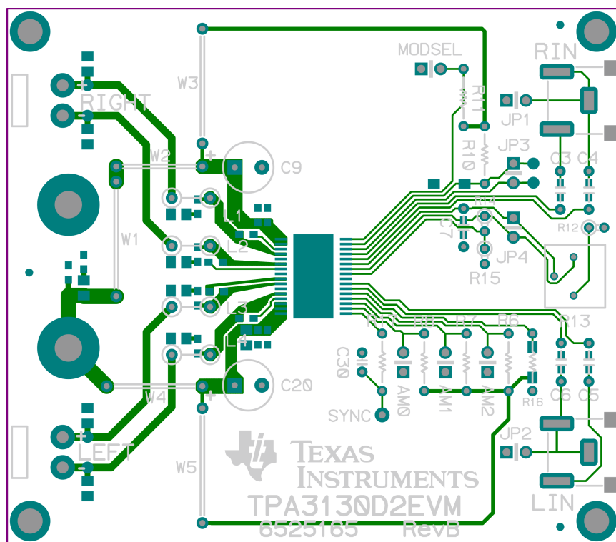
Figure 5. TPA3130D2EVM Top X-ray View
