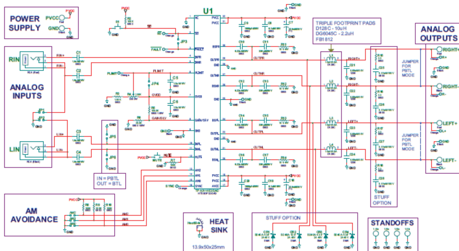
Figure 2. TPA3116D2EVM Schematic
