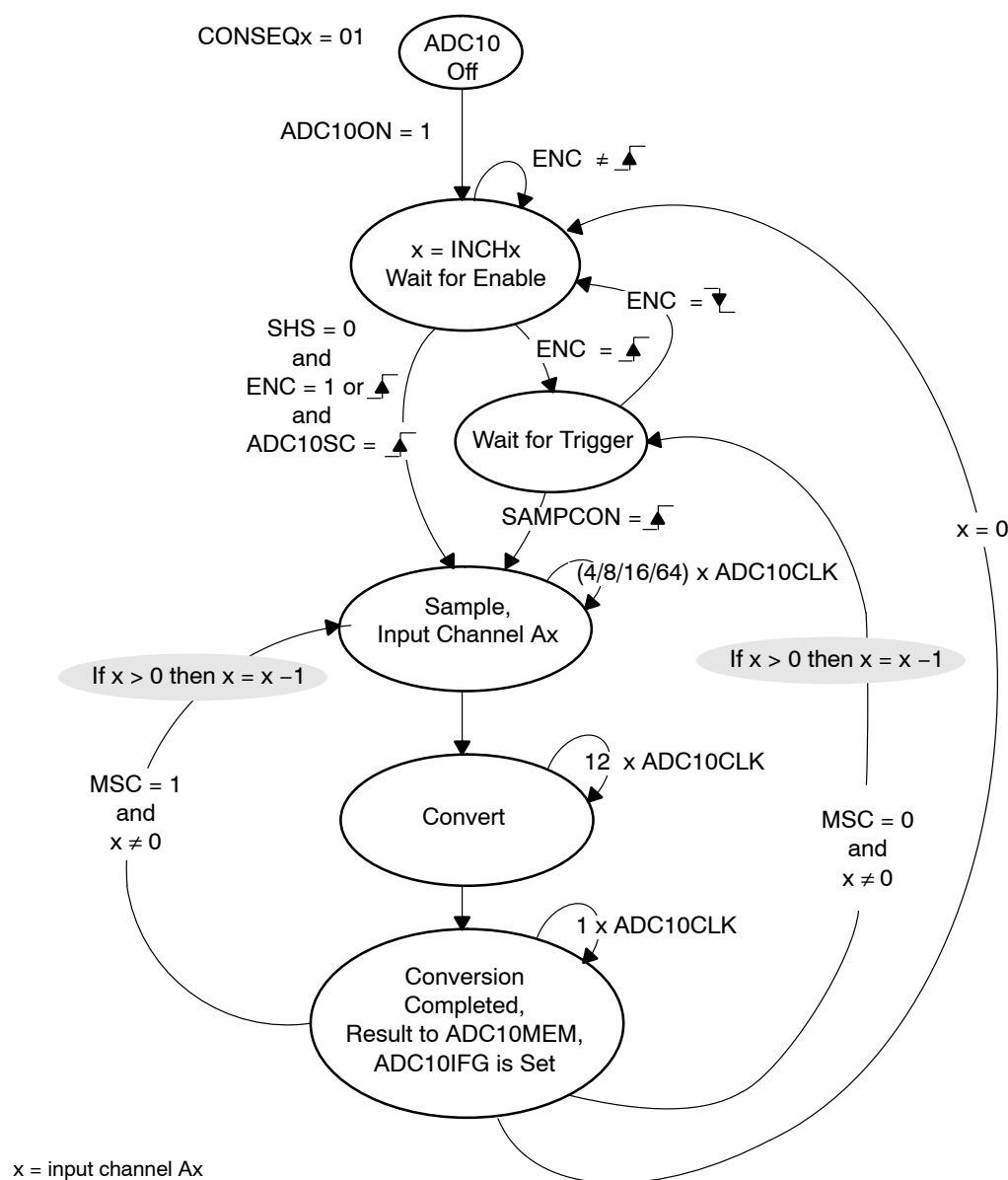
Figure 27–6. Sequence-of-Channels Mode
