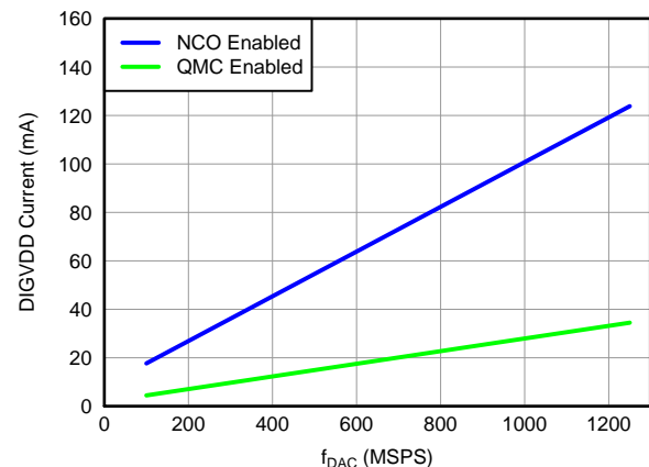
Figure 42. DIGVDD Current vs f_{DAC} Over Digital Processing Functions
