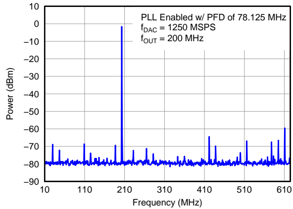
Figure 13. Single Tone Spectral Plot
