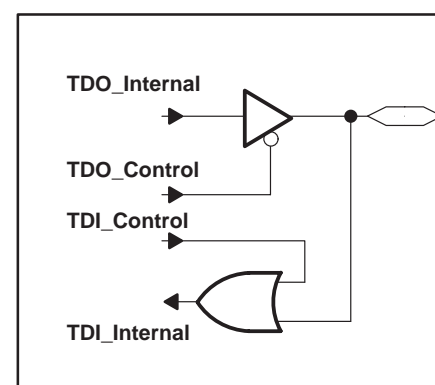
MSP430P/E325: TDO/TDI
