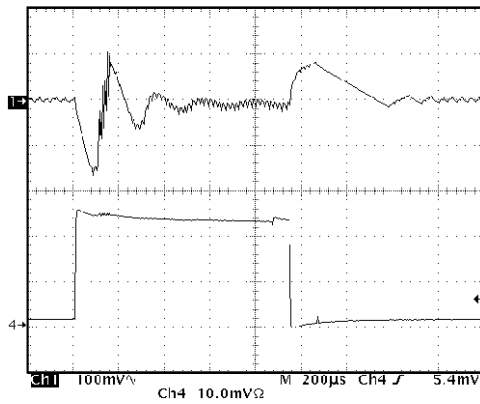
250 - mA Transient 12 V Converter (V IN = 10 V)
