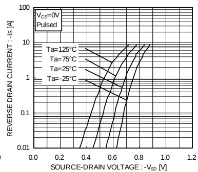
Fig.9 Reverse Drain Current vs. Source-Drain Voltage
