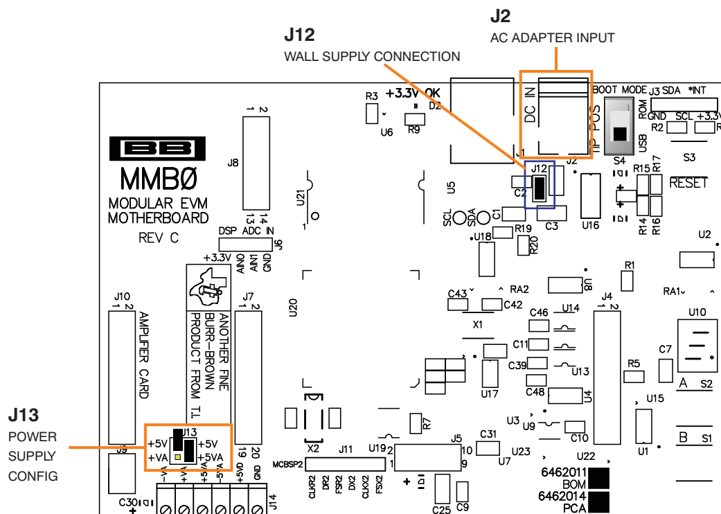
Figure 10. Connecting an AC Adapter
