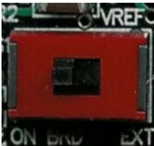
Figure 4. Switch S1
