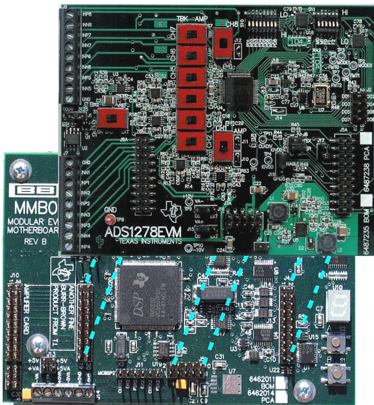
Figure 9. Connecting ADS1278EVM to MMB0
