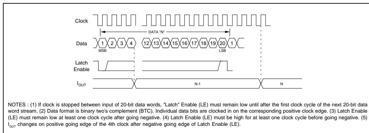
FIGURE 2. Timing Diagram.
