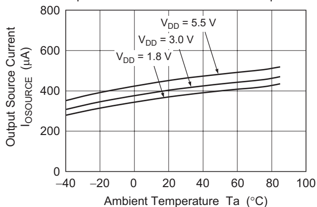
Figure 2-5. HA1630S05 Output Source Current vs. Ambient Temperature
