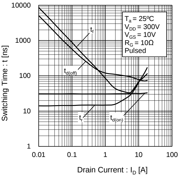
Fig.20 Switching Characteristics
