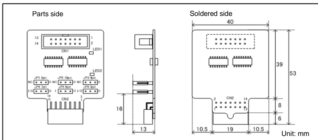
Figure 4.2 External Dimensions
