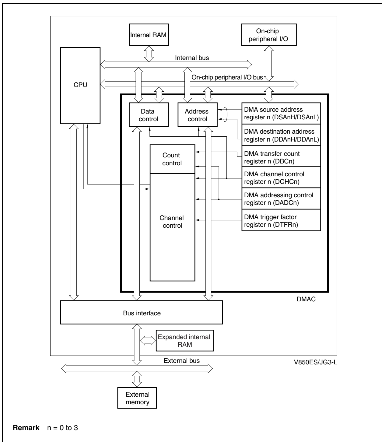
Figure 21-1. Block Diagram of DMAC
