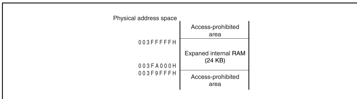
Figure 3-11. Expanded internal RAM (24 KB)
