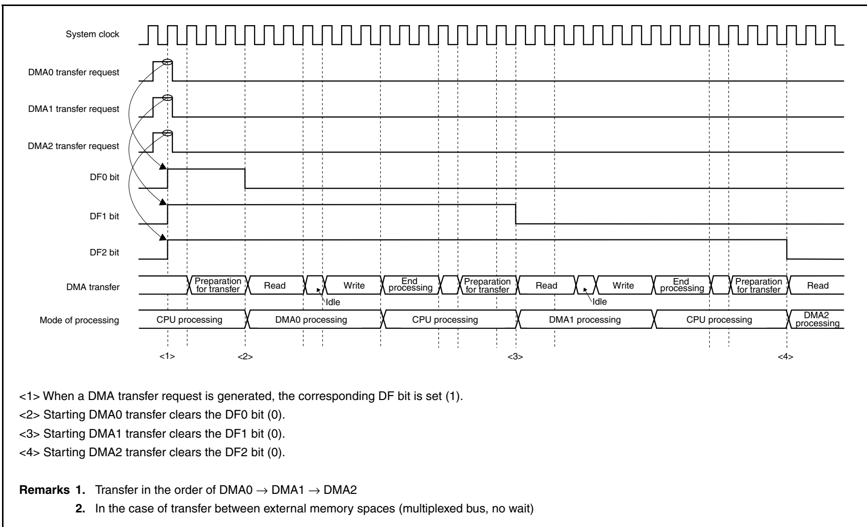
Figure 21-4. Priority of DMA (1)
