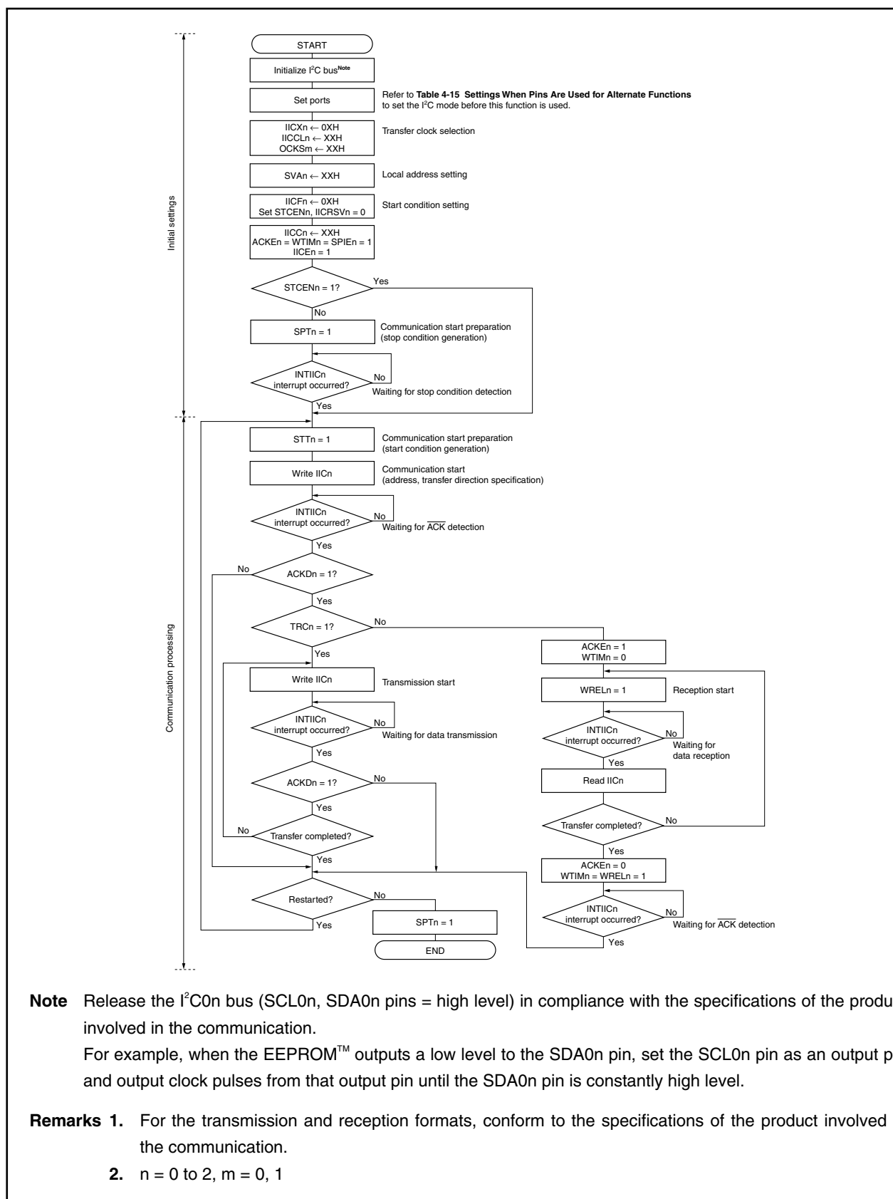
Figure 19-18. Master Operation in Single Master System
