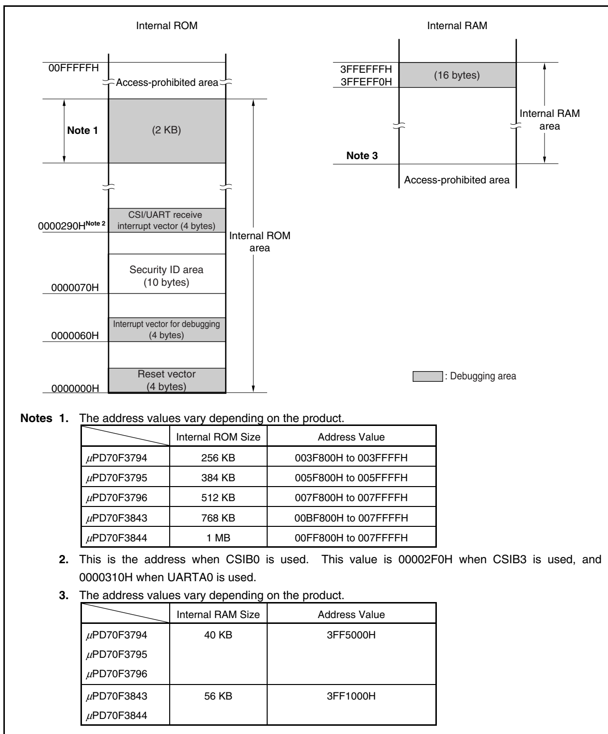
Figure 32-5. Memory Spaces Where Debug Monitor Programs Are Allocated
