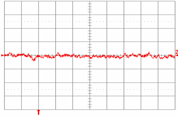
Fig. 1.0V.12: Input reflected ripple current, i_s ( 10\ \text{mA/div} ), measured through 10\ \mu\text{H} at the source at full rated load current and V_{in} = 48\ \text{V} . Refer to Fig. 1.0V.11 for test setup. Time scale: 1\ \mu\text{s/div} .
