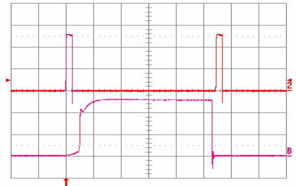
Fig. 1.0V.15: Load current (top trace, 20\ \text{A/div} , 20\ \text{ms/div} ) into a 10\ \text{m}\Omega short circuit during restart, at V_{in} = 48\ \text{V} . Bottom trace ( 20\ \text{A/div} , 1\ \text{ms/div} ) is an expansion of the on-time portion of the top trace.
