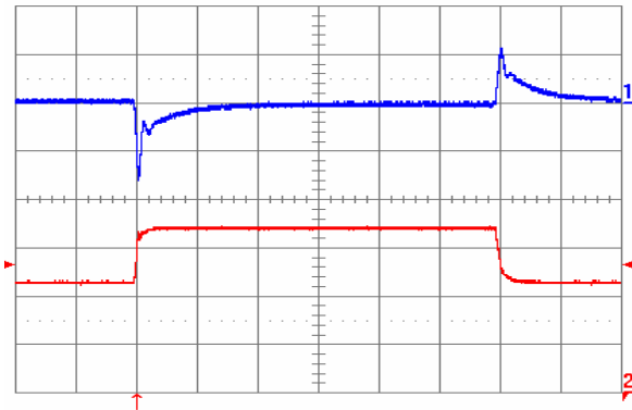
Fig. 1.8V.9: Output voltage response to load current step-change (22.5 A – 33.75 A – 22.5 A) at V_{in} = 48\text{ V} . Top trace: output voltage (100 mV/div.). Bottom trace: load current (10 A/div.). Current slew rate: 1 A/ \mu\text{s} . C_o = 470\text{ }\mu\text{F} tantalum + 1 \mu\text{F} ceramic. Time scale: 0.2 ms/div.
