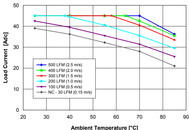
Fig. 2.5V.2: Available load current vs. ambient air temperature and airflow rates for QM48T45025 converter with B height pins mounted horizontally with V_{in} = 48\text{ V} , air flowing from pin 3 to pin 1, and MOSFET temperature \leq 120^\circ\text{C} .
