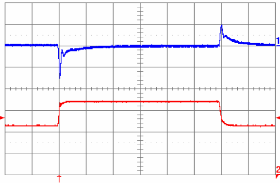
Fig. 2.5V.9: Output voltage response to load current step-change (22.5 A – 33.75 A – 22.5 A) at V_{in} = 48 V. Top trace: output voltage (100 mV/div.). Bottom trace: load current (10 A/div.). Current slew rate: 1 A/ \mu s. C_o = 470 \mu F tantalum + 1 \mu F ceramic. Time scale: 0.2 ms/div.
