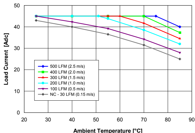
Fig. 1.8V.1: Available load current vs. ambient air temperature and airflow rates for QM48T45018 converter with B height pins mounted vertically with V_{in} = 48\text{ V} , air flowing from pin 3 to pin 1, and MOSFET temperature \leq 120^\circ\text{C} .
