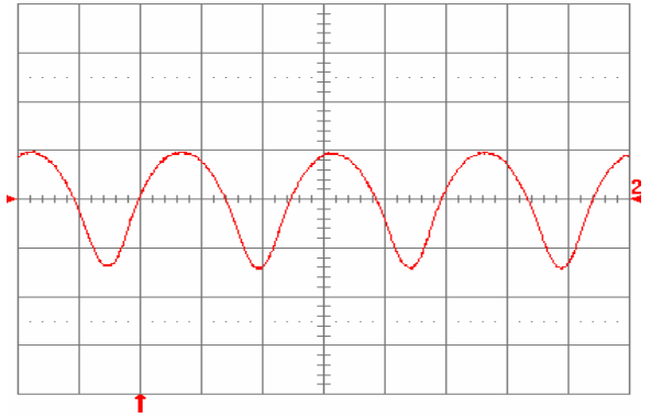
Fig. 1.0V.13: Input reflected ripple current, i_c ( 100\ \text{mA/div} ), measured at input terminals at full rated load current and V_{in} = 48\ \text{V} . Refer to Fig. 1.0V.11 for test setup. Time scale: 1\ \mu\text{s/div} .
