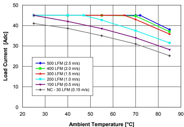
Fig. 2.0V.2: Available load current vs. ambient air temperature and airflow rates for QM48T45020 converter with B height pins mounted horizontally with V_{in} = 48\text{ V} , air flowing from pin 3 to pin 1, and MOSFET temperature \leq 120^\circ\text{C} .
