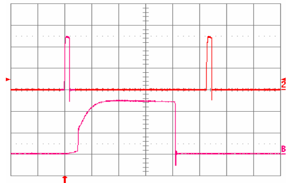
Fig. 1.8V.15: Load current (top trace, 20 A/div, 20 ms/div) into a 10 m\Omega short circuit during restart, at V_{in} = 48 V. Bottom trace (20 A/div, 1 ms/div) is an expansion of the on-time portion of the top trace.
