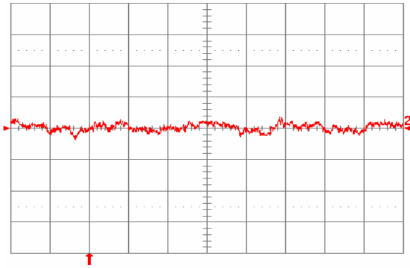
Fig. 3.3V.12: Input reflected ripple current, i_s (10 mA/div), measured through 10 µH at the source at full rated load current and V_{in} = 48 V. Refer to Fig. 3.3V.11 for test setup. Time scale: 1 µs/div.
