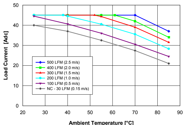
Fig. 2.5V.1: Available load current vs. ambient air temperature and airflow rates for QM48T45025 converter with B height pins mounted vertically with V_{in} = 48\text{ V} , air flowing from pin 3 to pin 1, and MOSFET temperature \leq 120^\circ\text{C} .
