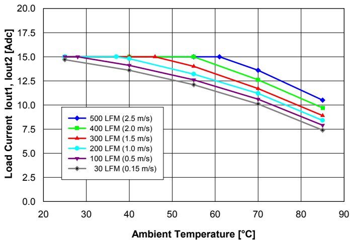
Fig. 14: Available balanced load current ( I_{out1} = I_{out2} ) vs. ambient air temperature and airflow rates for converter mounted vertically with V_{in} = 48\text{ V} , air flowing from pin 3 to pin 4 and maximum FET temperature \leq 120^{\circ}\text{C} .
