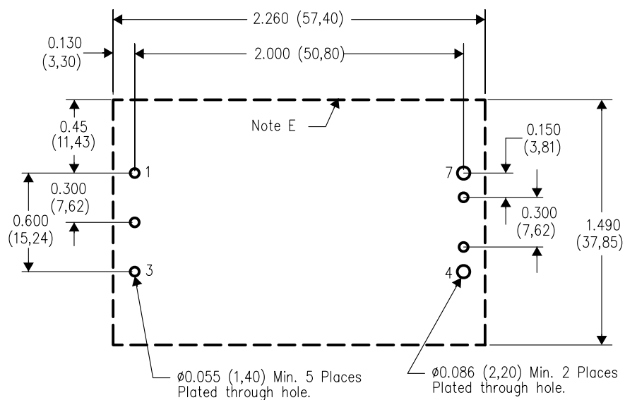
PCB Layout
