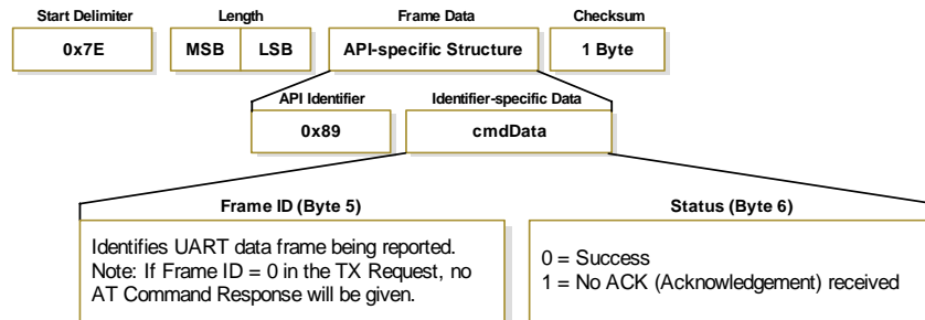
Figure 3-7. TX Status Frames
