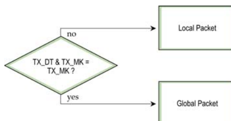
Figure 4-03. Address Recognition (@ the Transmitting RF Modem)
