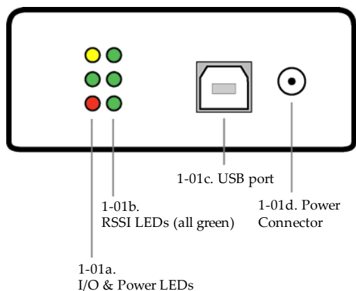
Figure 1-01. Front View
