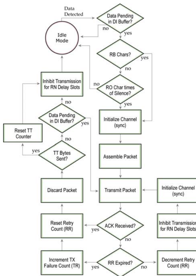
Figure 4-07. Acknowledged Mode State Diagram (TX modem)
