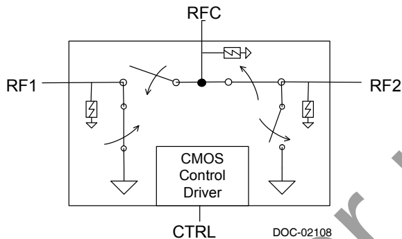
Figure 1. Functional Diagram
