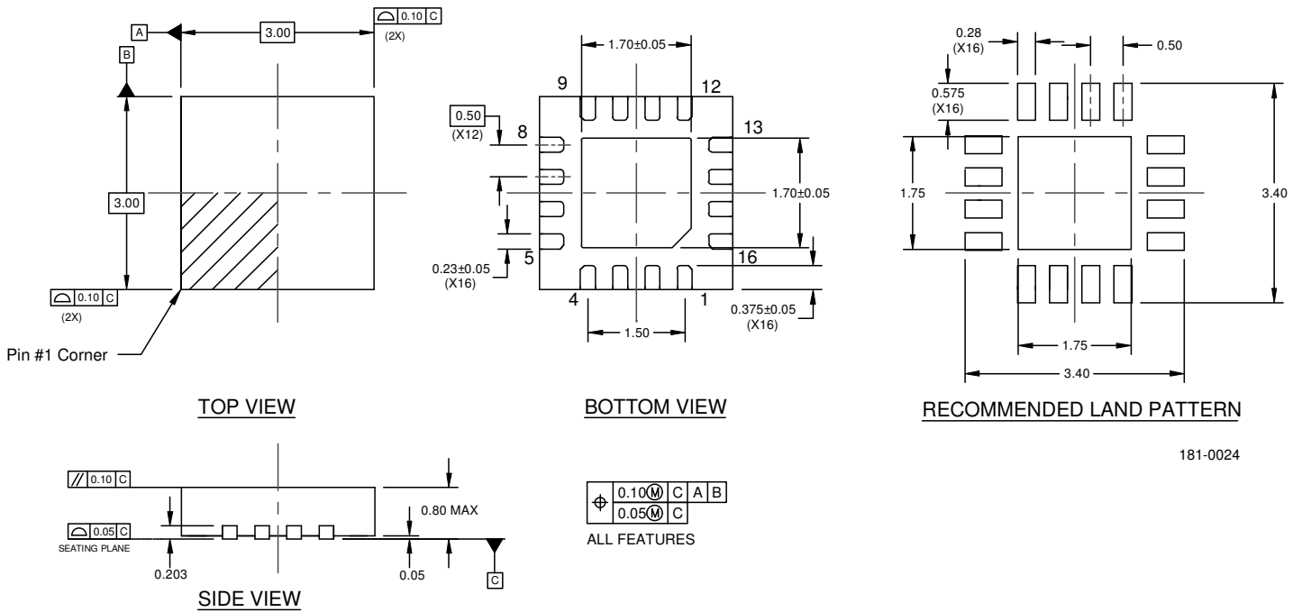
Figure 13. Package Drawing
