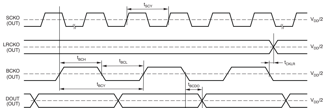
Figure 22. Latency Time Between Input Biphase and LRCKO/DOUT
