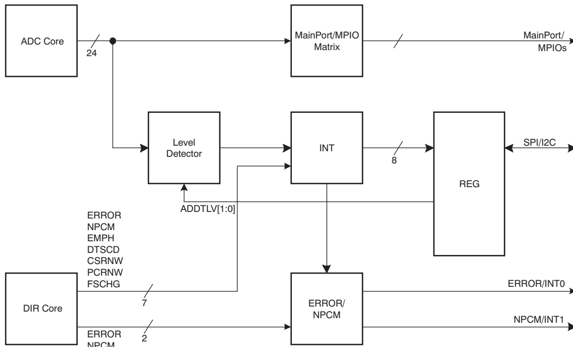
Figure 18. Block Diagram for ADC Level Detection
