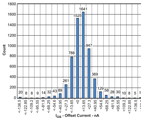
Figure 50. Input Offset Current
