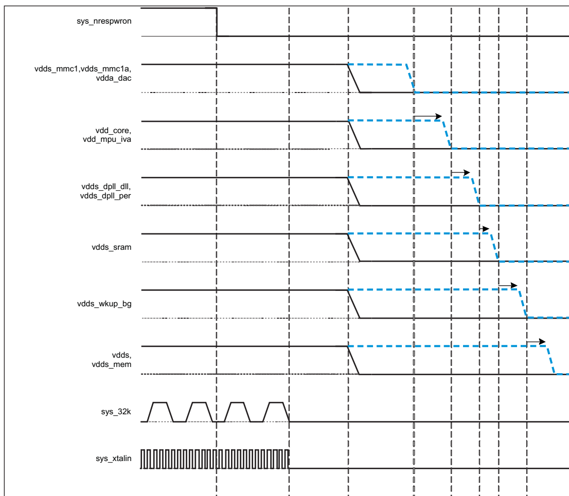
Figure 3-4. Power-down Sequence
