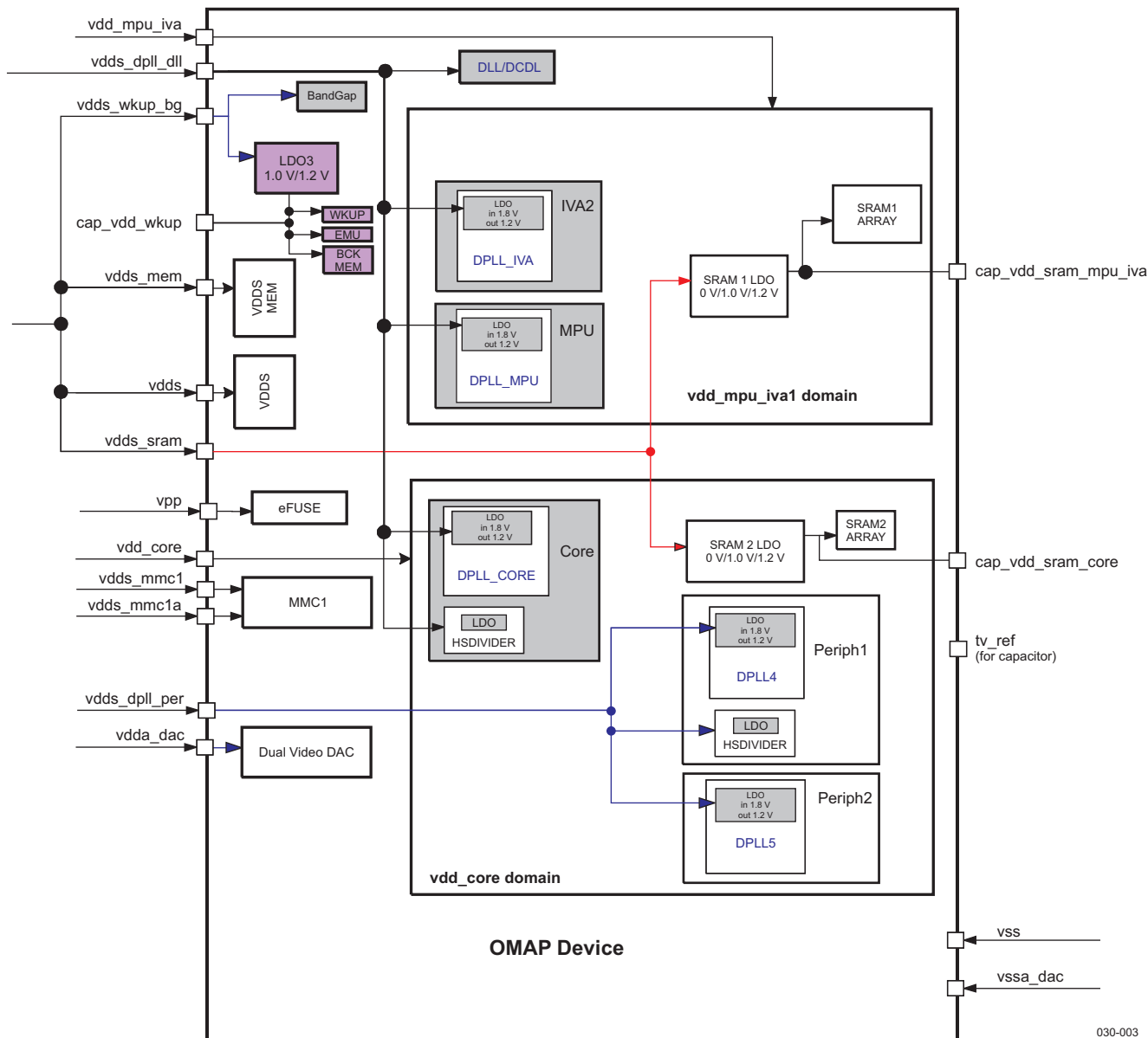
Figure 3-1. OMAP3525 and OMAP3530 Power Domains
