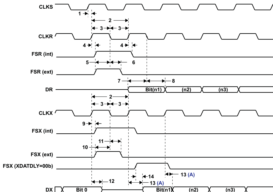
Figure 5-33. McBSP Timing
