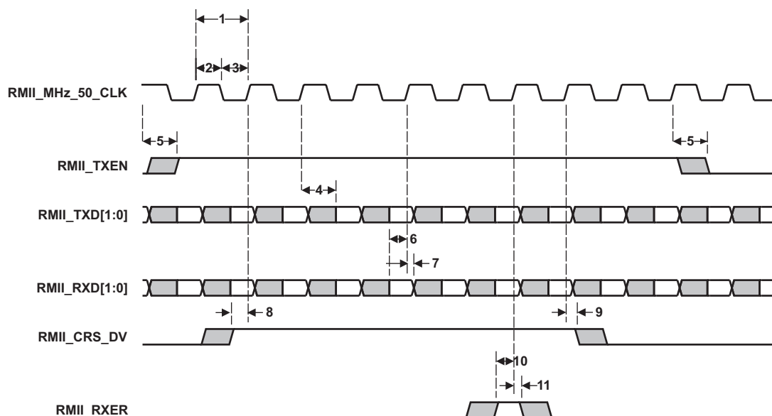
Figure 5-50. RMII Timing Diagram
