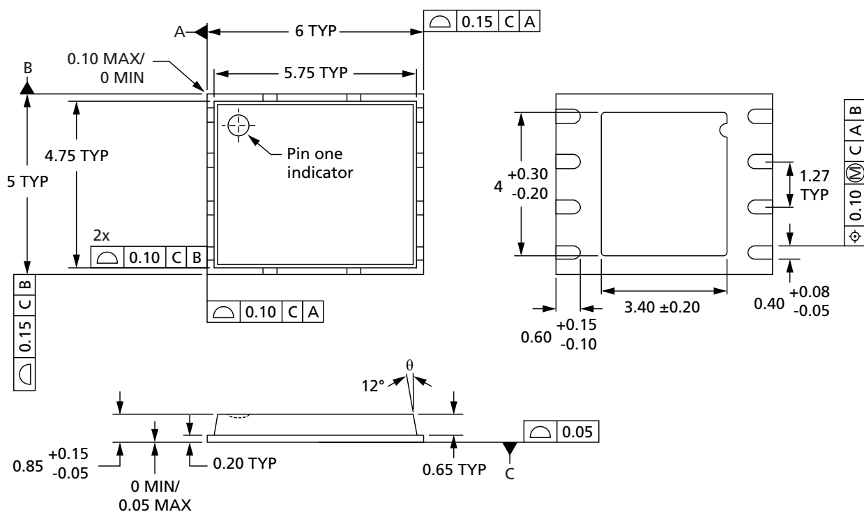
Figure 42: V-PDFN-8 6mm x 5mm (MLP8) – Package Code: F6
