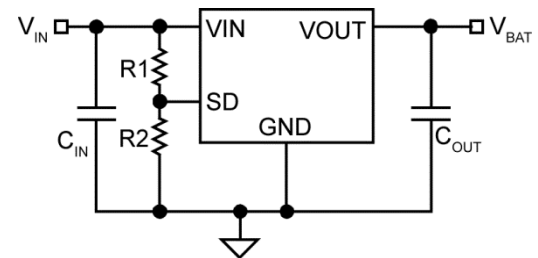
Figure 7. Auto-Shutdown using Shutdown Pin
