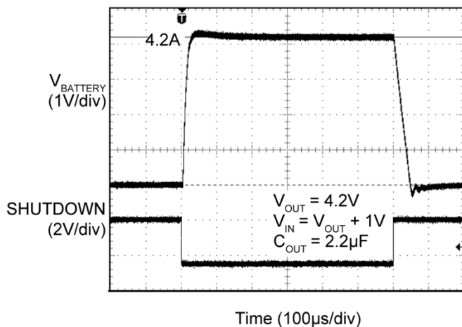
Shutdown Transient
