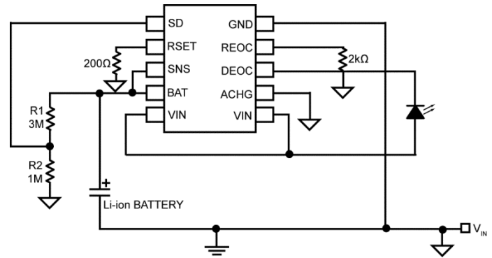
Figure 6. Top-Off Charger with Internal Reset – Application Circuit
