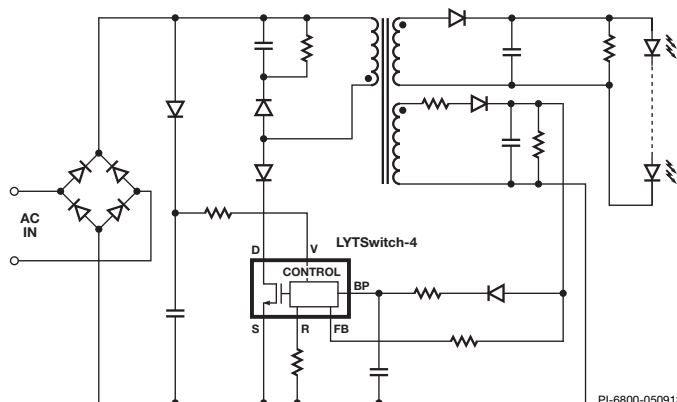
Figure 1. Typical Schematic.
