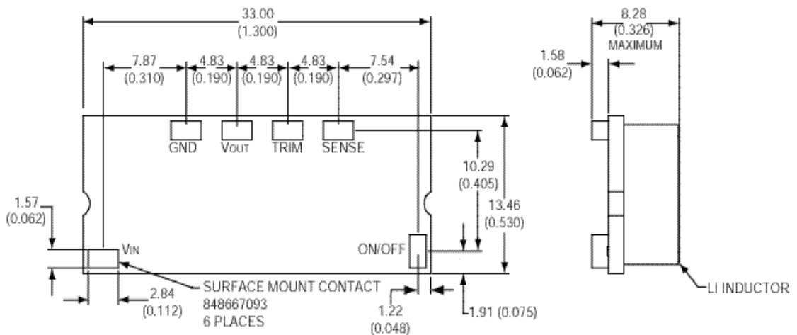
SIDE VIEW
