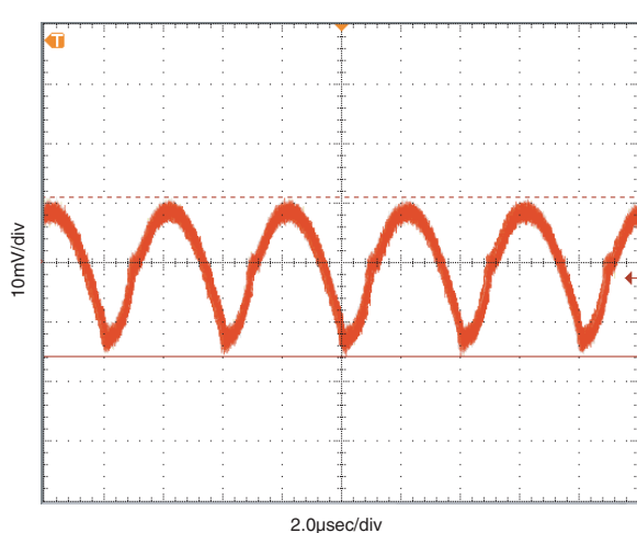
Output Ripple Noise ( V_{IN} = 12V , V_{OUT} = 2.5V , I_{OUT} = 10A , C_{OUT} = 10\mu F Tantalum || 1 \mu F ceramic)
