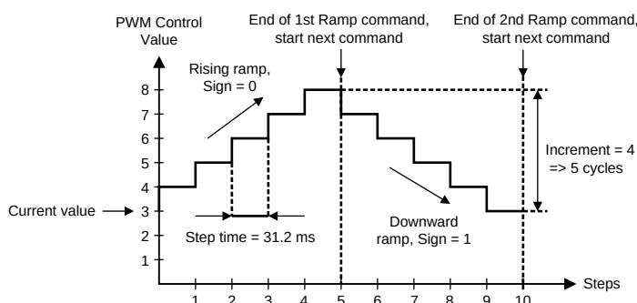
Figure 18. Example of 2 sequential ramp commands
