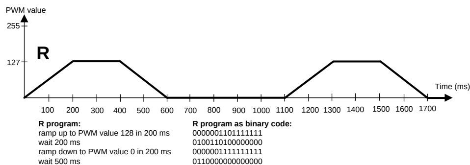
Figure 34. Sequence diagram
