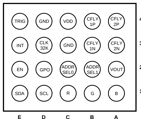
Figure 3. Bottom View
