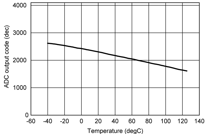
Figure 23. LP3925 ADC Temperature Range
