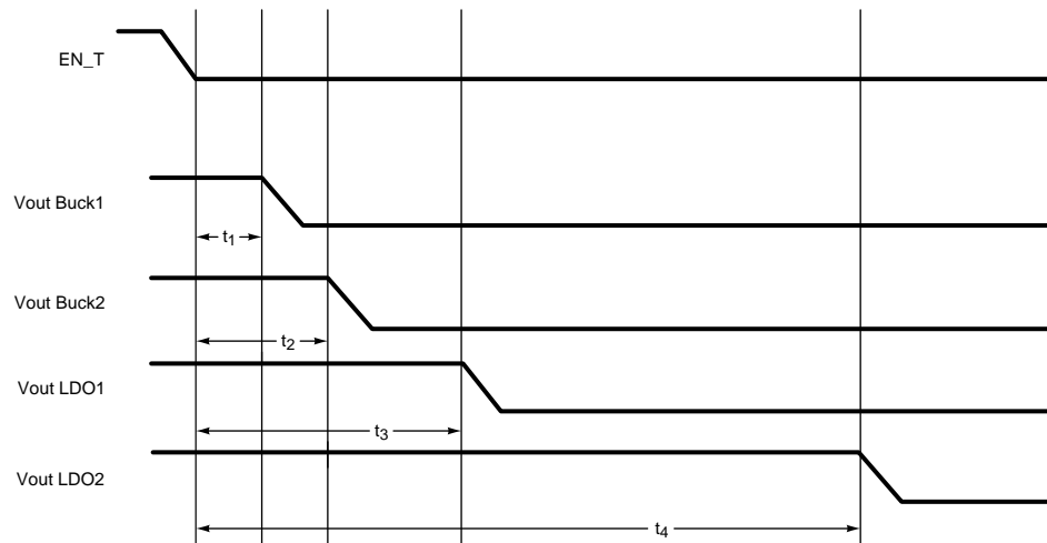
Figure 36. LP3907 Default Power-On Sequence
