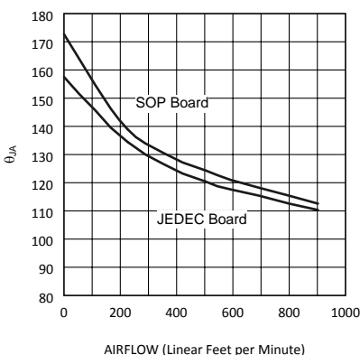
Figure 21. \theta_{JA} vs Airflow (SOIC-8)
