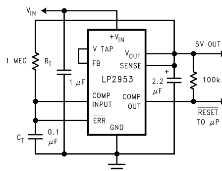
Figure 44. 5V Regulator with Timed Power-On Reset
