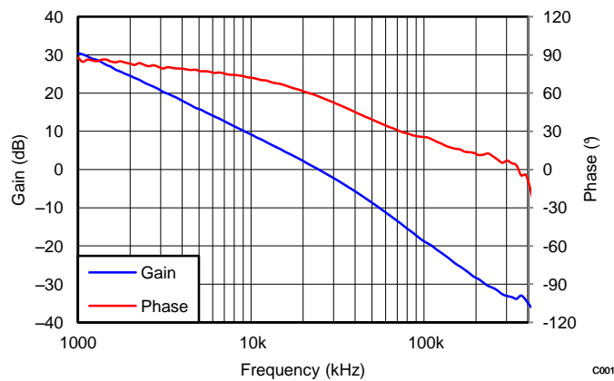
Figure 16. V OUT = 1.8 V, I OUT = 4 A, C OUT = 200 μF ceramic, f SW = 500 kHz
