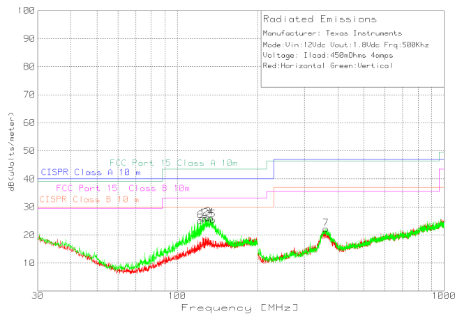
Figure 48. Radiated Emissions 12-V Input, 1.8-V Output, 4-A Load (EN55022 Class B)
