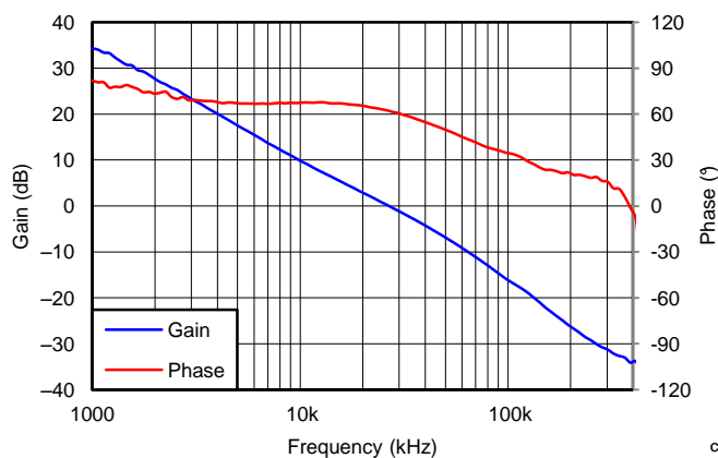
Figure 11. V OUT = 1.8 V, I OUT = 4 A, C OUT = 200 \mu F ceramic, f SW = 500 kHz
