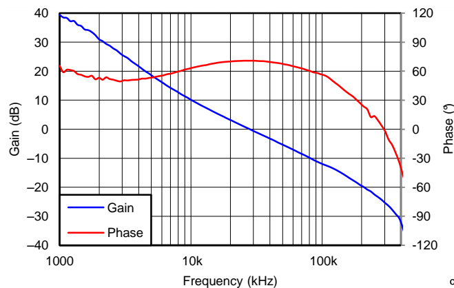
Figure 6. V OUT = 1.8 V, I OUT = 4 A, C OUT = 200 µF ceramic, f SW = 500 kHz
