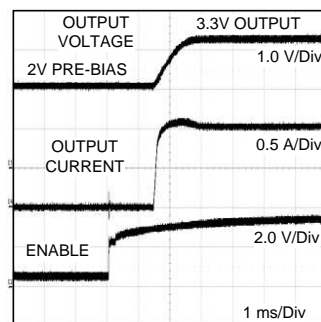
Figure 35. Pre-Biased Startup
