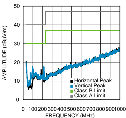
Figure 4. Radiated EMI (EN 55022) V_{IN} = 24V , V_{OUT} = 5V , I_{OUT} = 10A
