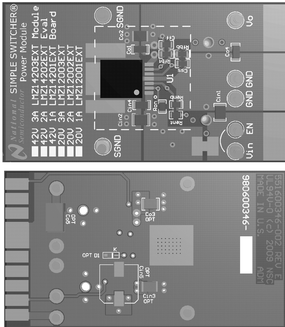
Figure 43. Top And Bottom View Of Evaluation PCB
