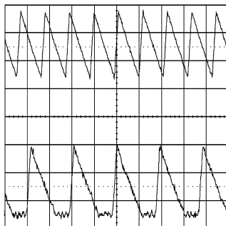
Figure 40. CCM and DCM Operating Modes V_{IN} = 12V, V_O = 3.3V, I_O = 1A/0.25A
