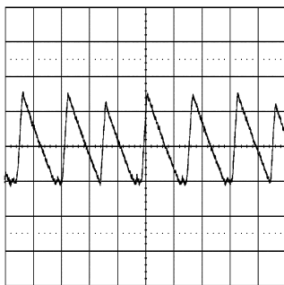
Figure 41. Transition Mode Operation V_{IN} = 12V, V_O = 3.3V, I_O = 0.29A
