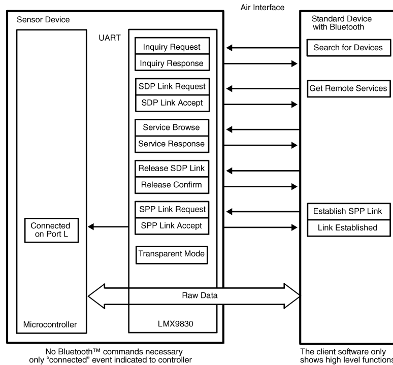
Figure 24. Point-to-Point Connection
