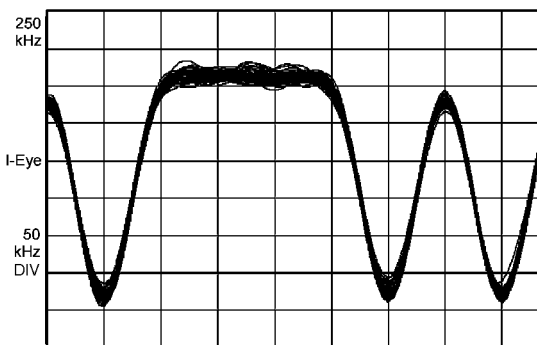
Figure 2. Modulation
