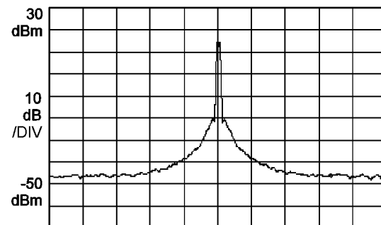
Figure 3. Transmit Spectrum
