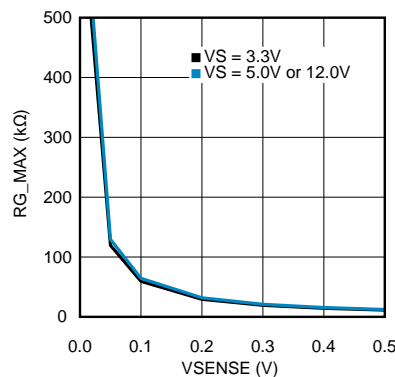
Figure 29. Allowed R G for CASE 1
