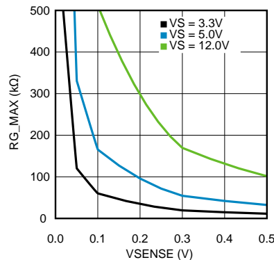
Figure 31. Allowed R_G for CASE 3
