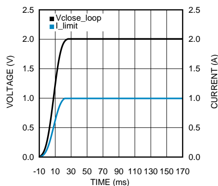
Figure 37. Plot for the Resistive Load Application with the LP38501 LDO Regulator
