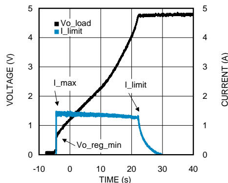
Figure 33. SuperCap Application with LM3102 Regulator Plot
