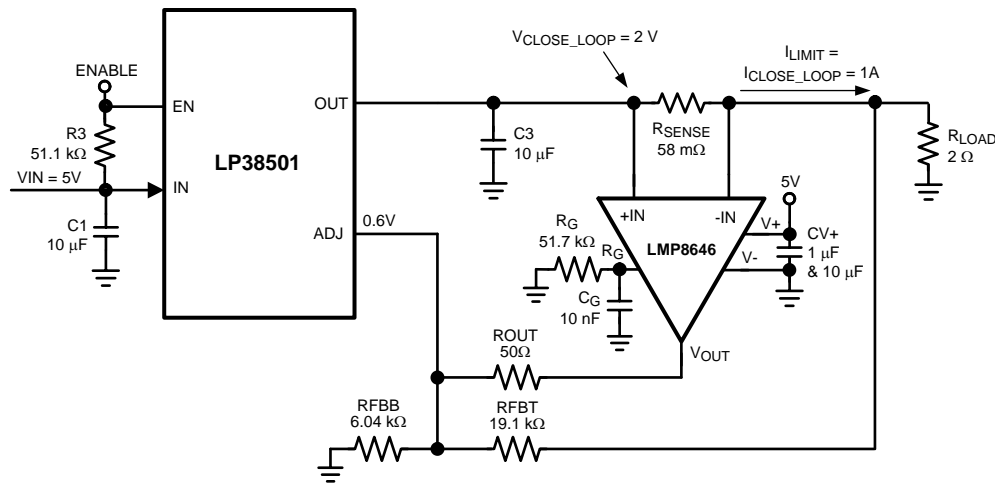
Figure 36. Resistive Load Application with LP38501 Regulator
