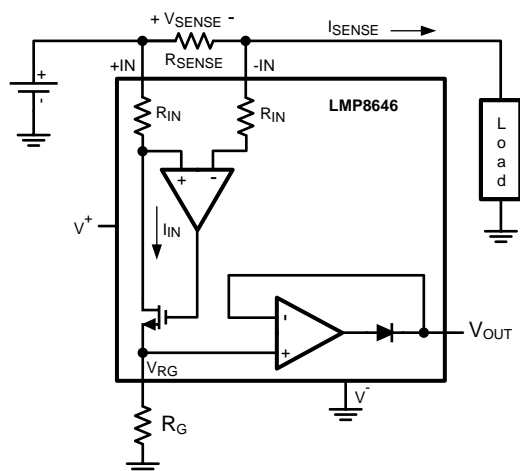
Figure 27. Current Monitor
