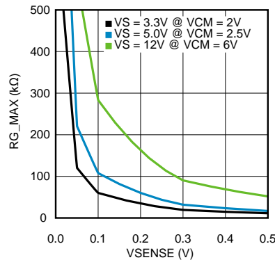
Figure 30. Allowed R_G for CASE 2
