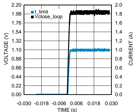
Figure 35. Plot for the Resistive Load Application with LMZ12003 Regulator Plot
