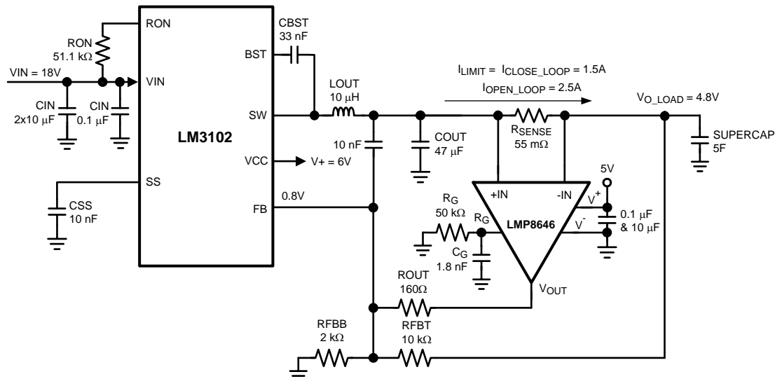
Figure 32. SuperCap Application with LM3102 Regulator
