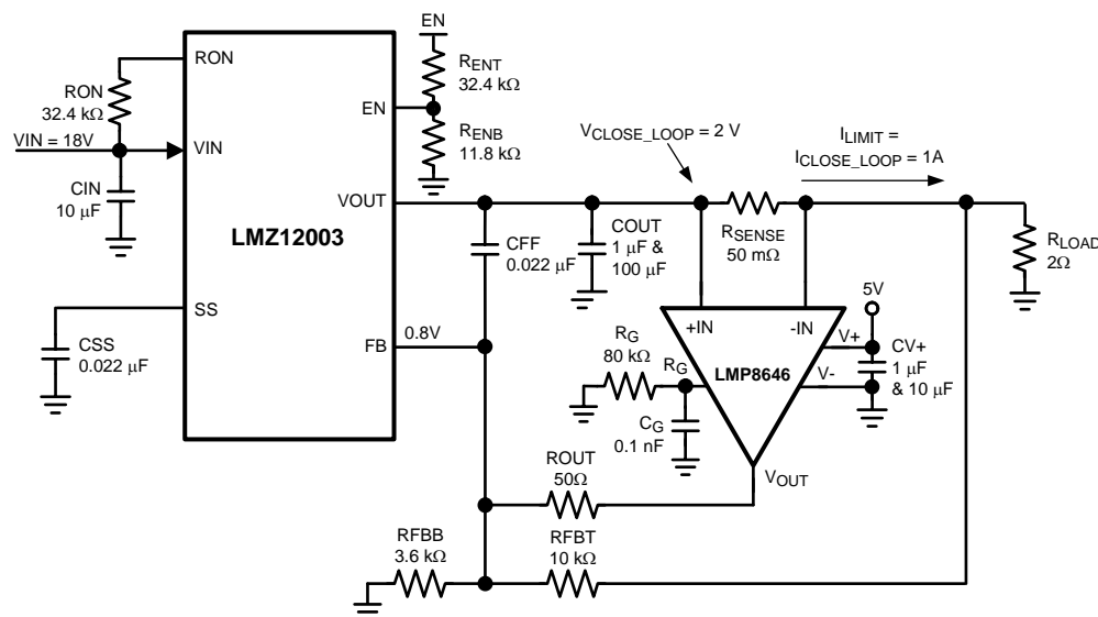
Figure 34. Resistive Load Application with LMZ12003 Regulator
