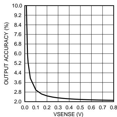
Figure 28. Output Accuracy vs. V_{\text{SENSE}}
